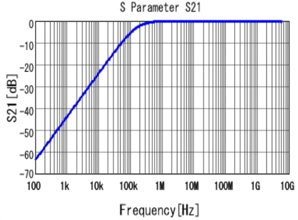
■ GCJ188R71E103KA01 S21 DCOV, 25degC
