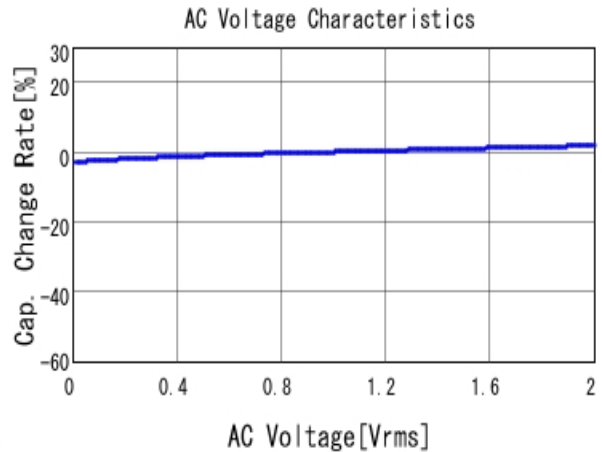
■ GCJ188R71E103KA01 C-AC Voltage capchange, DCOV, 25.0d
