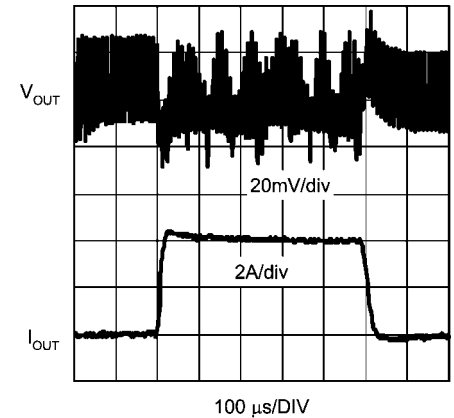
Load Transient Response V_{CC} = 3.3V, V_{IN} = 5V, V_{REF} = 0.6V, V_{OUT} = 1.2V C_{SS} = 12nF, F_{SW} = 300kHz
