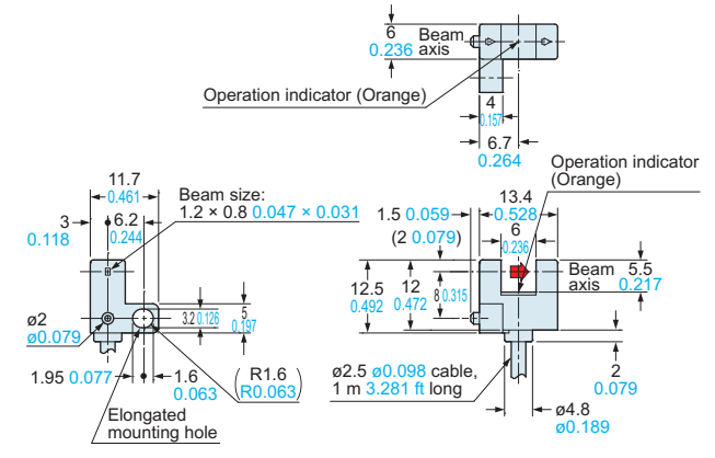
PM-F25 Sensor
