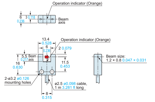
PM-U25 Sensor
