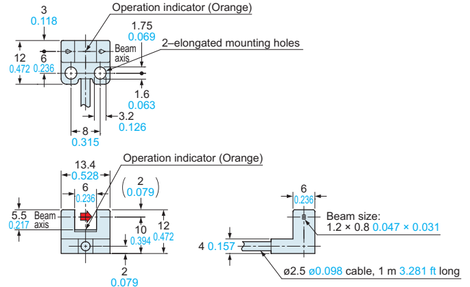
PM-L25 Sensor
