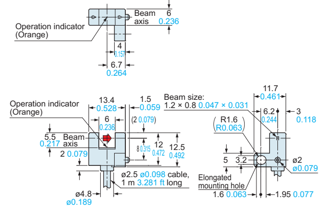
PM-R25 Sensor
