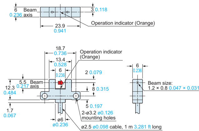
PM-K25 Sensor
