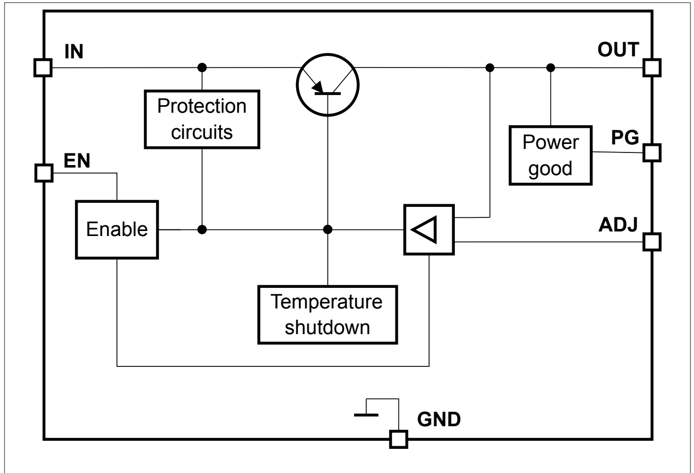
Figure 1 Block diagram
