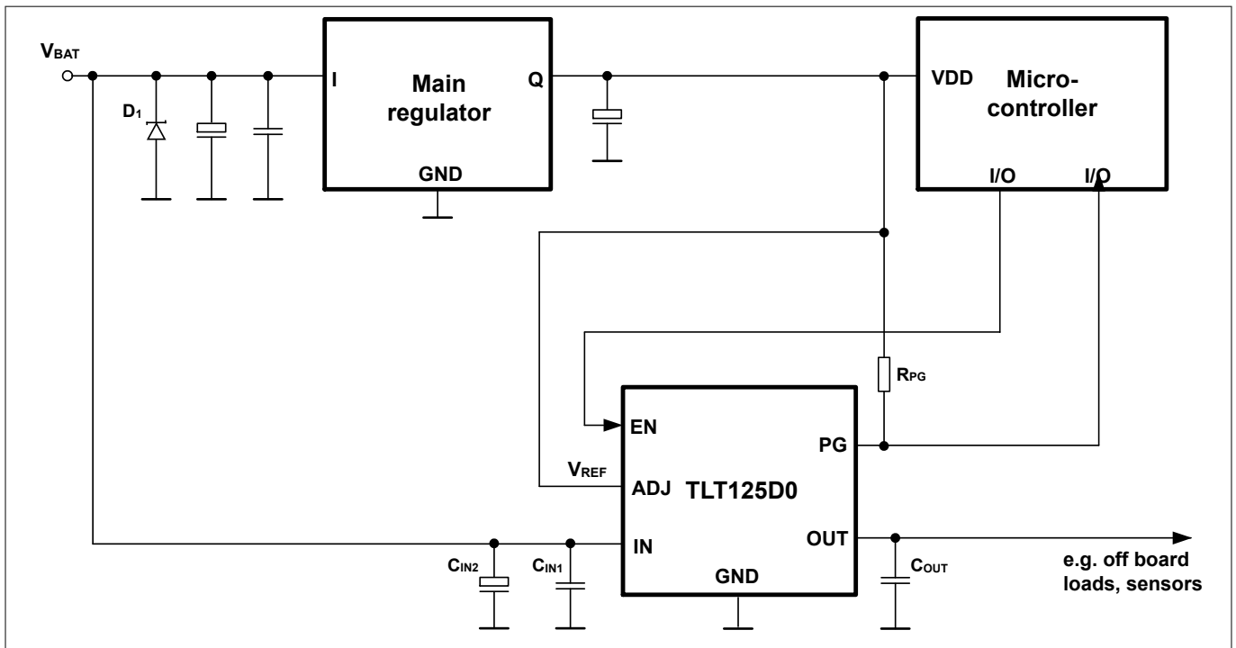
Figure 3 Application diagram
