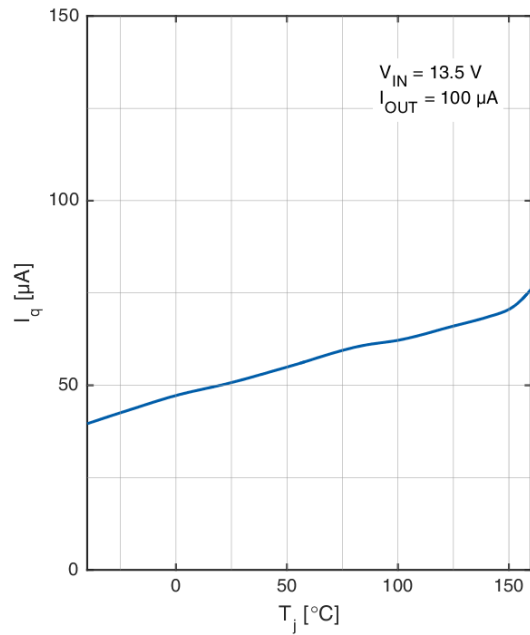
Current consumption I_q versus junction temperature T_j ( I_{OUT} low)
