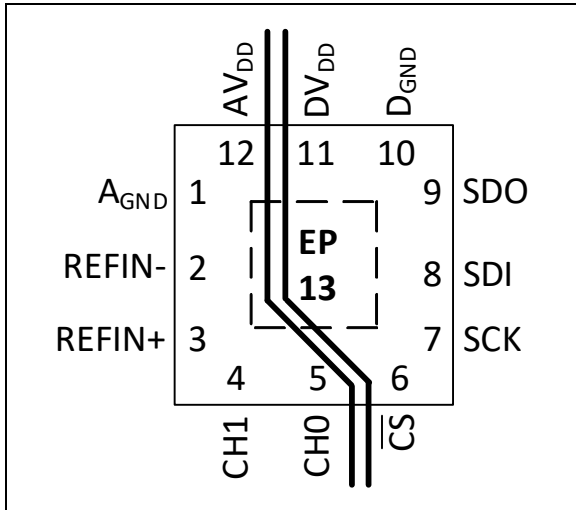
FIGURE 7-7: Separation of Analog and Digital Circuits on the Layout (Shown on the UQFN Package).
