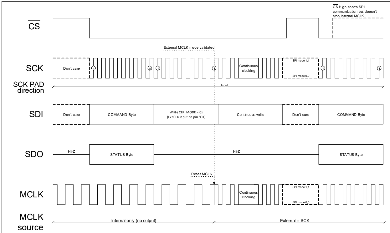
FIGURE 6-13: MCP3565R Transition from CLK_SEL[1:0] = 10 to 0x.
