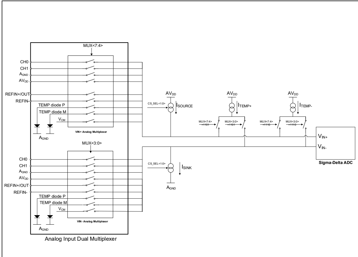
FIGURE 5-1: Simplified Analog Input Multiplexer Schematic.
