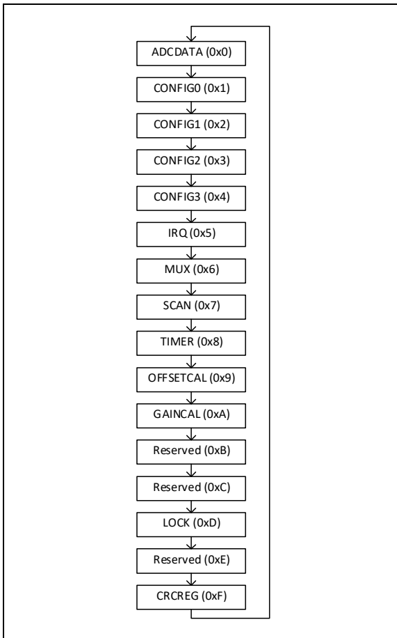
FIGURE 6-6: Incremental Read Loop.
