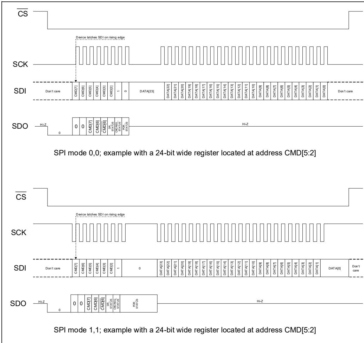
FIGURE 6-4: Single Register Write Communication (CMD[1:0] = 10) Timing Diagram.
