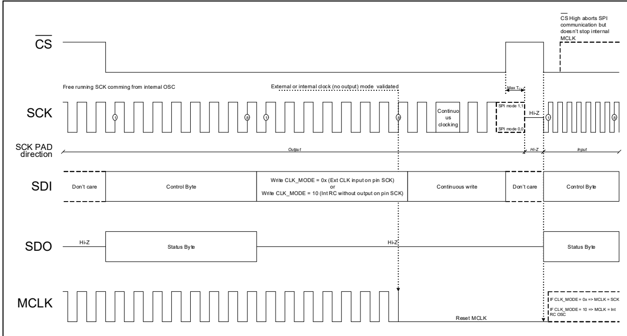
FIGURE 6-16: MCP3565R Transition from CLK\_SEL[1:0] = 11 to 0x/10 .
