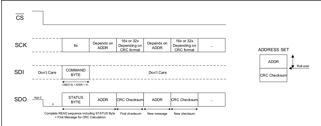
FIGURE 6-11: SPI Static Read with Communication CRC Enabled.
