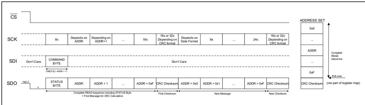
FIGURE 6-12: SPI Incremental Read with Communication CRC Enabled.
