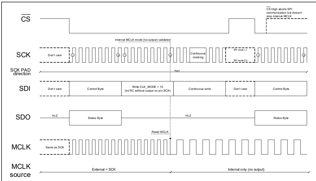
FIGURE 6-14: MCP3565R Transition from CLK_SEL[1:0] = 0x to 10.
