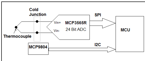
FIGURE 7-2: Thermocouple Connection.
