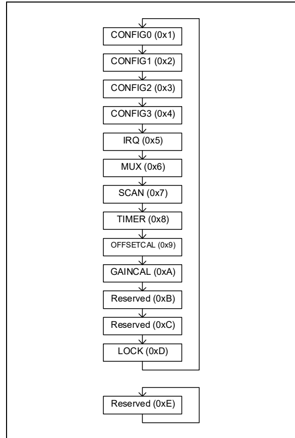
FIGURE 6-3: Incremental Write Loop.
