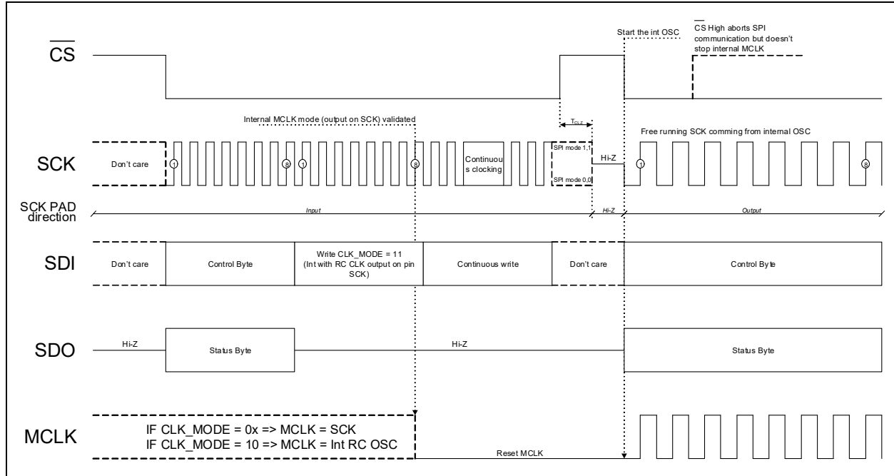
FIGURE 6-15: MCP3565R Transition from CLK_SEL[1:0] = 0x/10 to 11.
