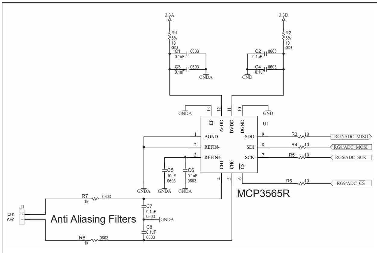
FIGURE 7-1: MCP3565R Application Example.
