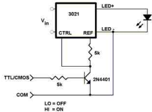
Figure 14. Pulse/Strobe input 5V=ON
