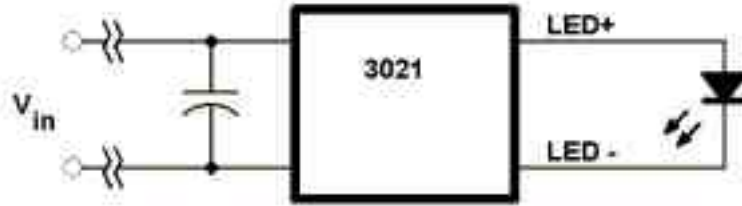
Figure 17. Place a capacitor across the input terminals when the distance to the DC power source is greater than 18 inches DO NOT USE A CAPACITOR WHEN USING AC POWER!
