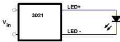
Figure 7. 700mA unit driving one Luxeon® V emitter (VIN ≥ 12VDC)
