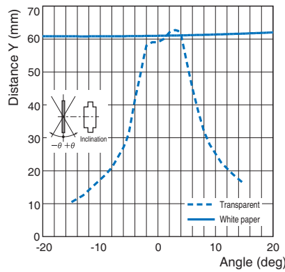
B5W-LB2112/LB2114/LB2122
