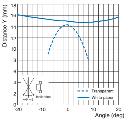
B5W-LB1
