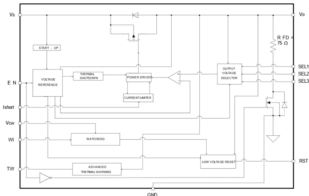
Figure 2. Functional block diagram of L99VR01J
