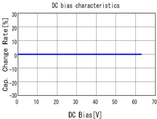
GCM1885C1J222JA16 C-DC bias capchange, 25.0degC, AC1V
