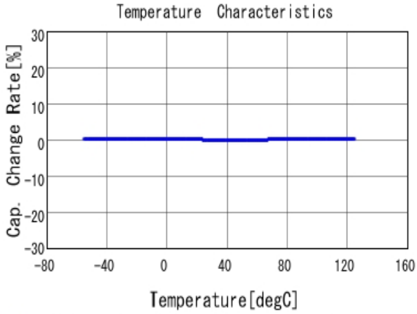
■ GCM1885C1J222JA16 C-Temp. capchange, DCOV, AC1Vrms
