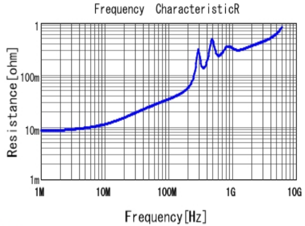
GCM1885C1J222JA16 R DCOV, 25degC
