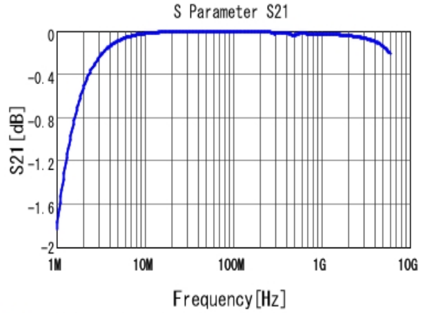
■ GCM1885C1J222JA16 S21 DCOV, 25degC
