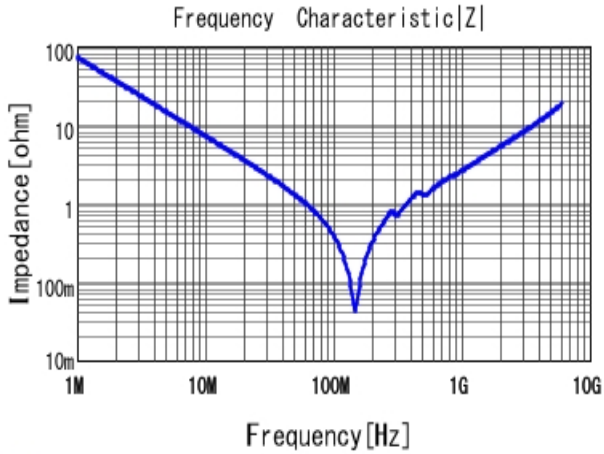
GCM1885C1J222JA16 |Z| DCOV, 25degC
