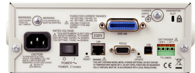
1908 rear panel (Protective buffer removed) GPIB optional.
