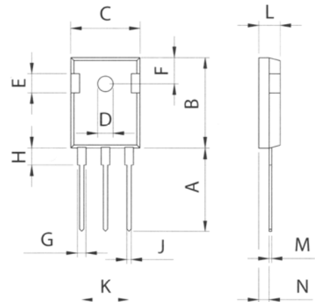
TO-247 AD
