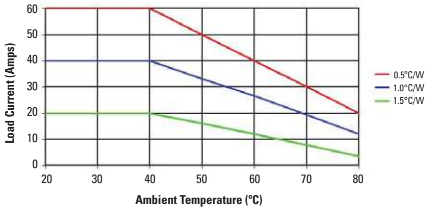
DP Series Derating Curve
