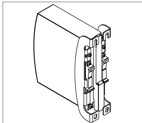
Fig. 21-4 Wall mounting with DIN rail brackets*)
