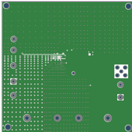
Figure 3—Inner Layer 1
