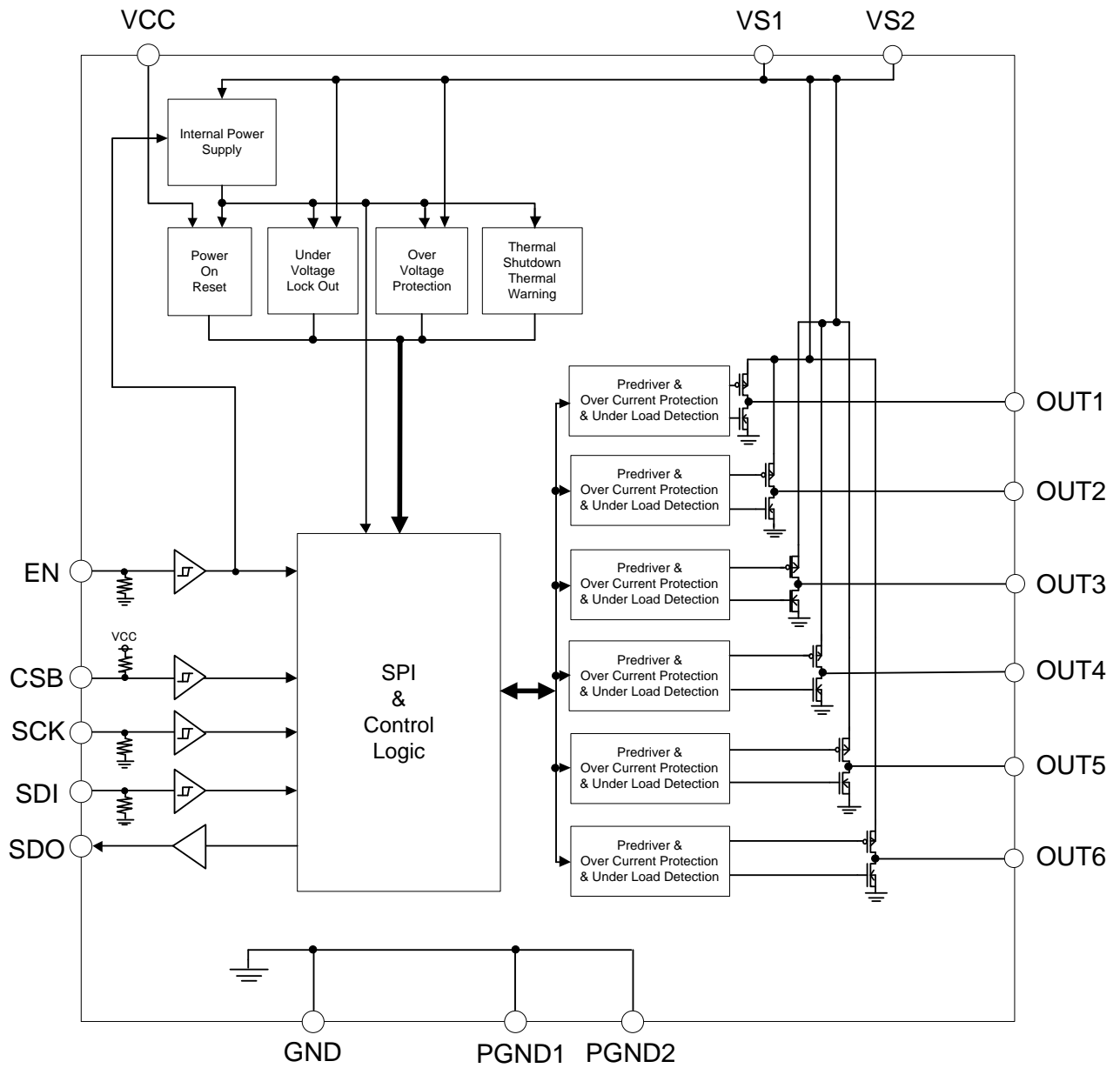
Figure 3. Block Diagram
