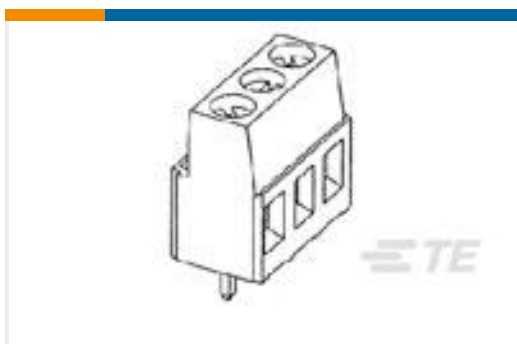
TE Part #1-796949-8 18POS TERMI-BLOK PCB MOUNT
