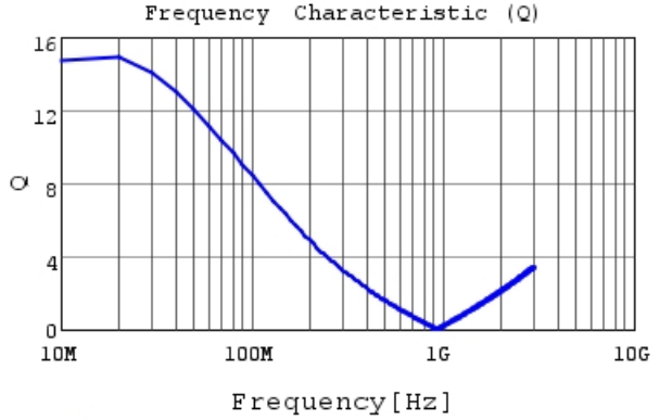
LQW18CNR65J0H Q
