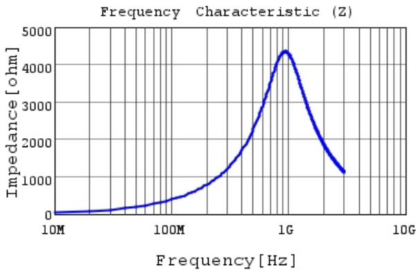
LQW18CNR65J0H |Z|
