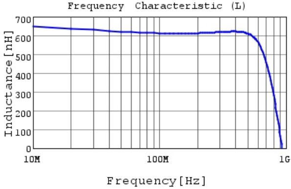
LQW18CNR65J0H L
