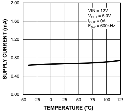
VIN Operating Supply Current vs. Temperature (MIC28304-1)
