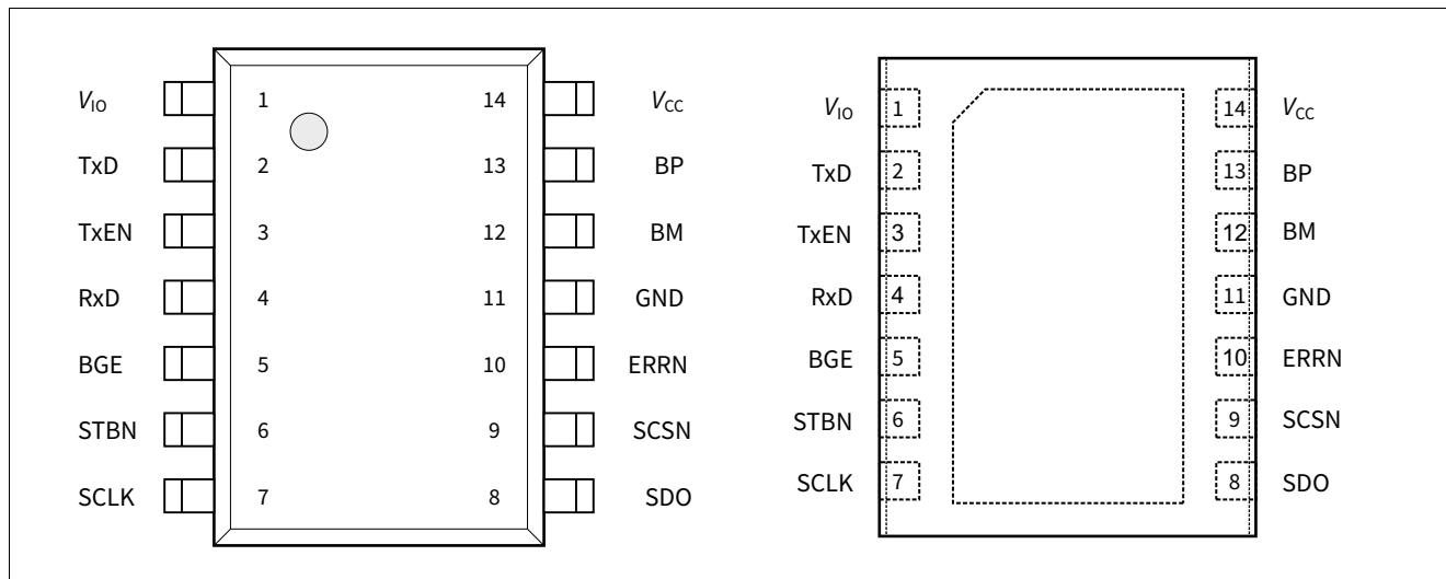
Figure 2 Pin configuration
