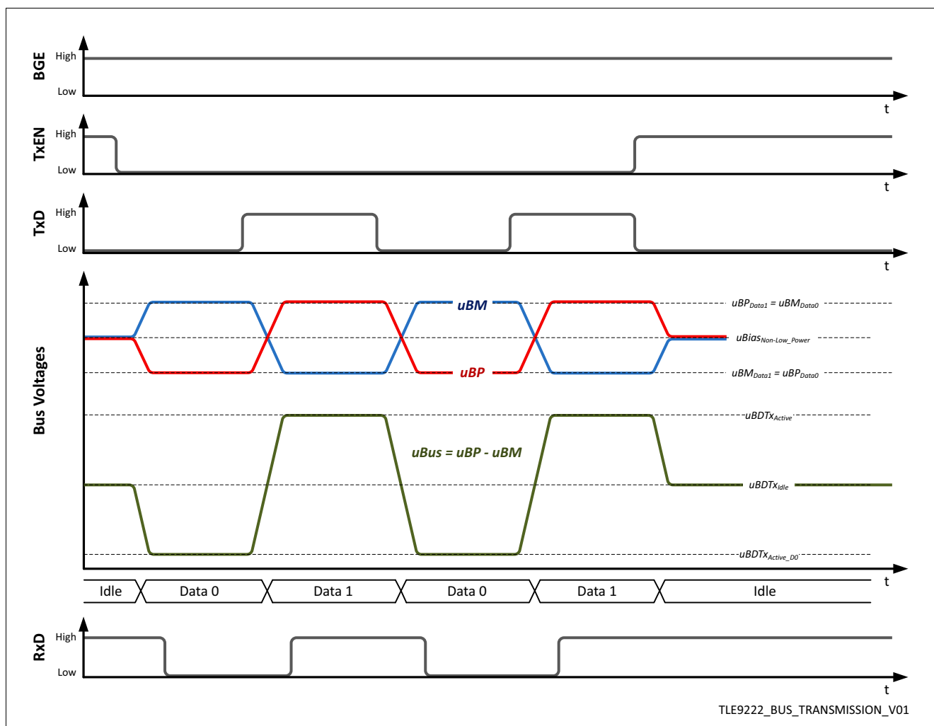
Figure 4 FlexRay physical layer bus signals
