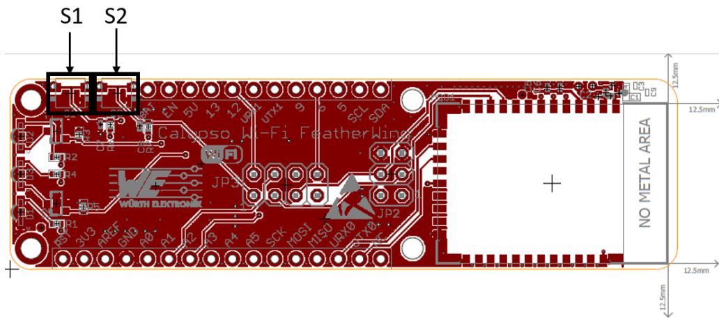
Figure 4: Push buttons
