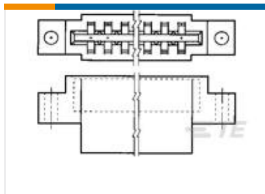
TE Part #1-583859-3 HOUSING CSTL 156 C/L 6 POS
