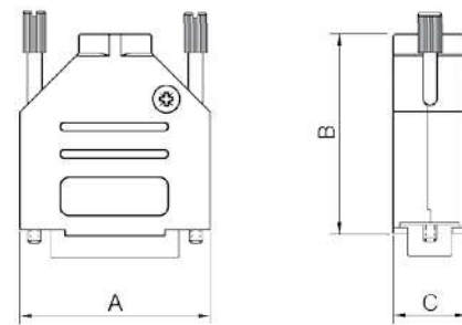
D-Sub-Hood
