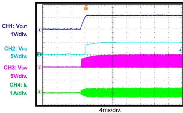
Power Good On I_{OUT} = 0A
