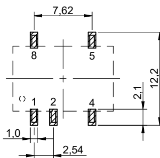
Figure 25: Recommended landpattern dimensions.
