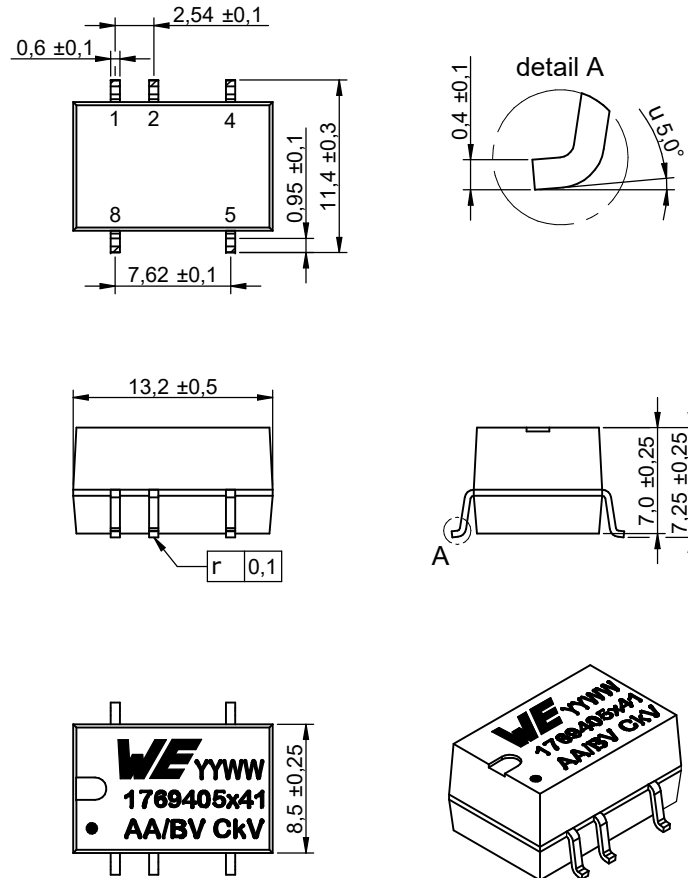
Figure 24: Physical dimensions.
