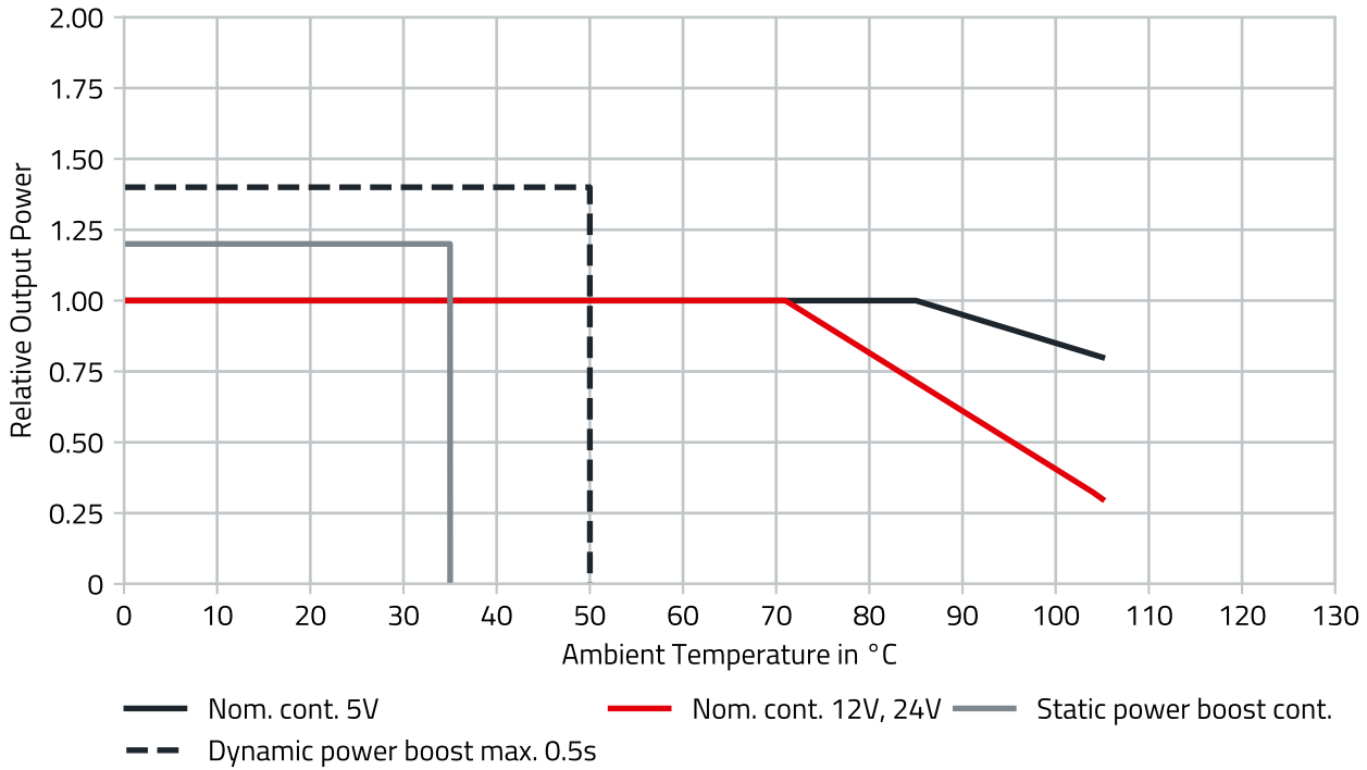
Figure 12: 1769405x41 power boost thermal derating nominal V IN .
