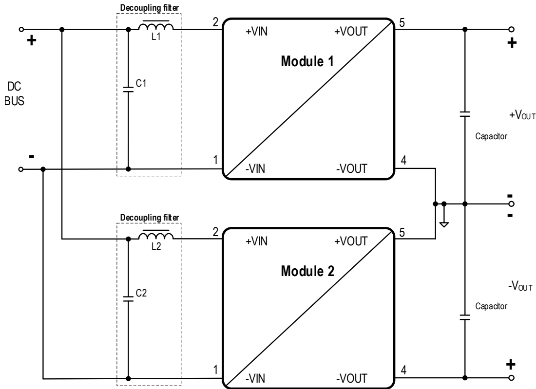
Figure 21: Generating complementary output voltages.
