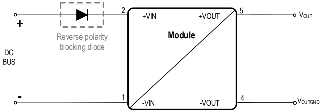
Figure 22: Reverse polarity protection.
