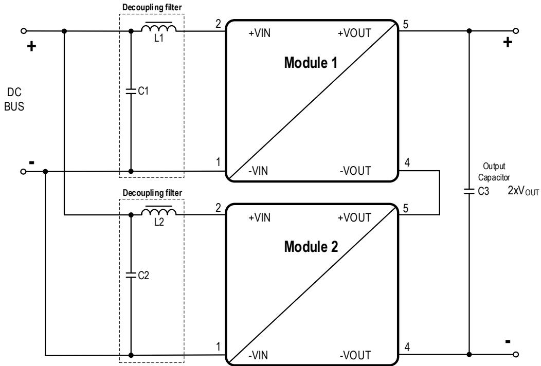
Figure 20: Primary side serial connection.
