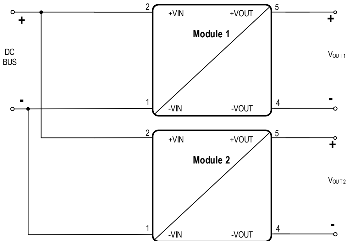
Figure 18: Primary side parallel connection.
