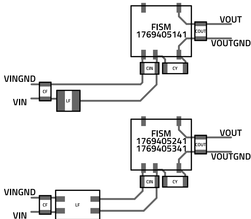
Figure 16: 1769405x41 layout recommendation.
