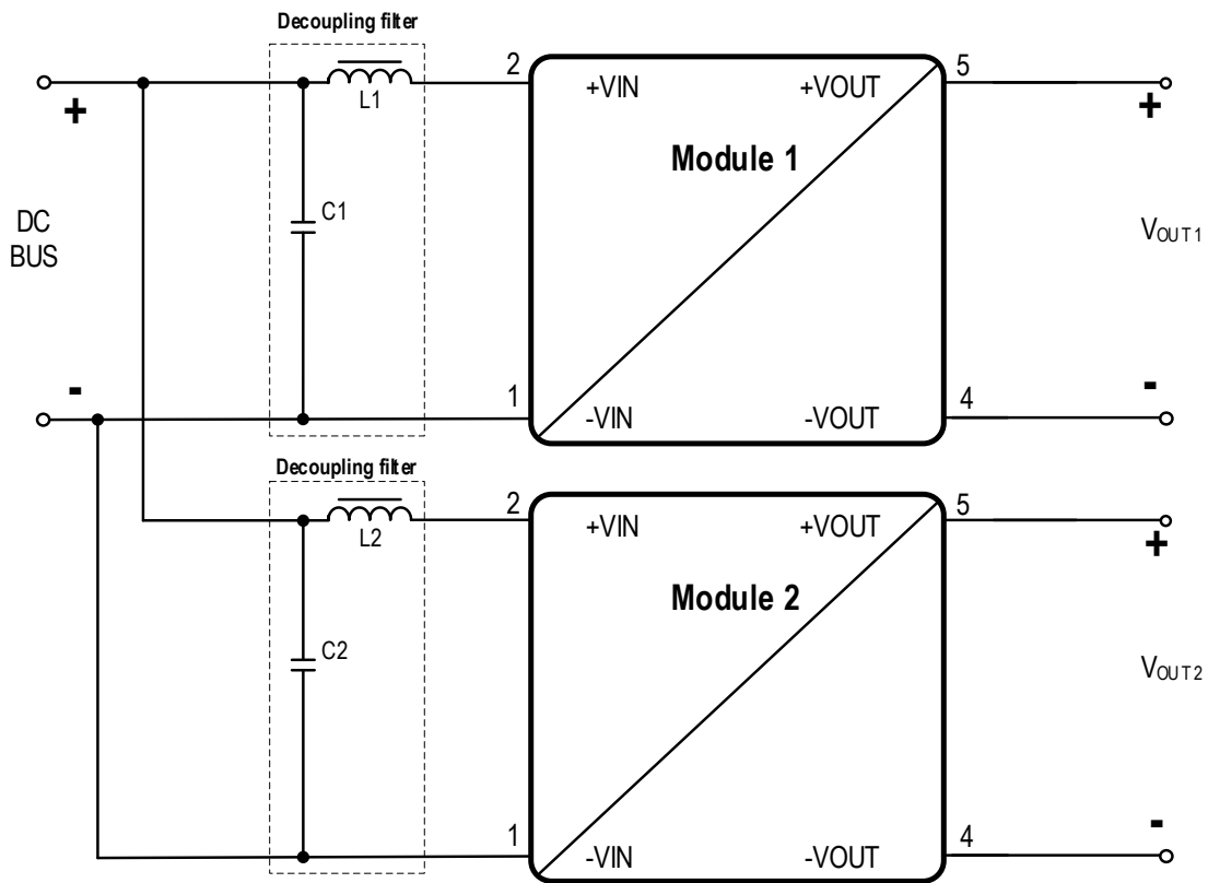
Figure 19: Decoupling for primary side parallel connection.
