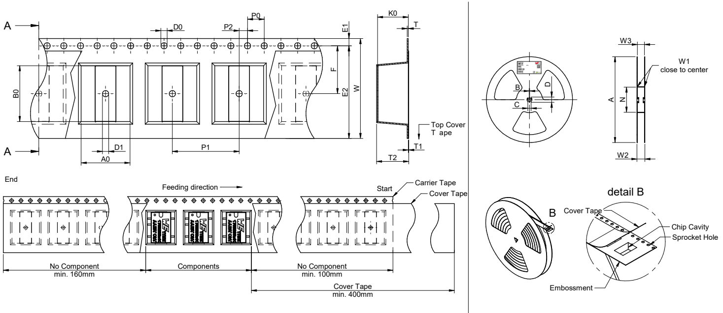
Figure 26: Packaging dimensions.
