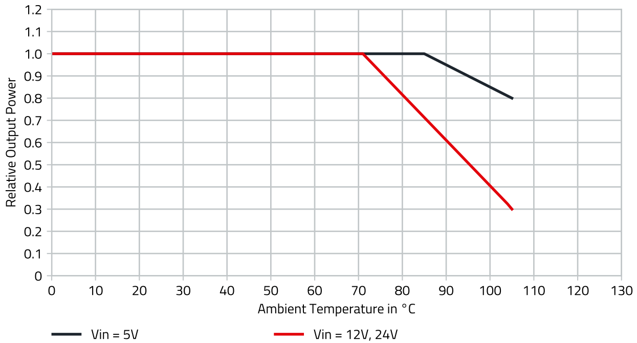
Figure 10: 1769405x41 output power thermal derating nominal V_{IN} , I_{OUT} = 0.4A .
