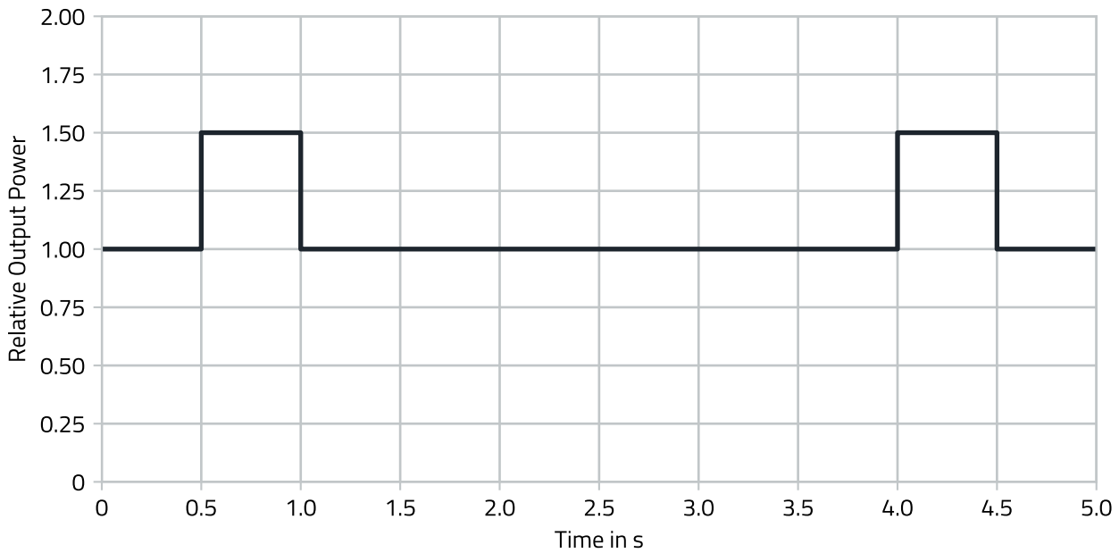
Figure 11: 1769405x41 dynamic power boost nominal V_{IN} , T_A = 25^\circ\text{C} .
