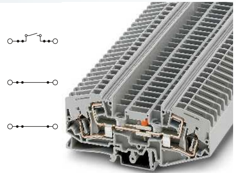
45 A, Messwandler-Trennklempen
