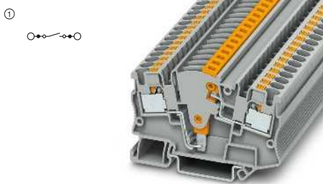
24 A, Messwandler-Trennklemme
