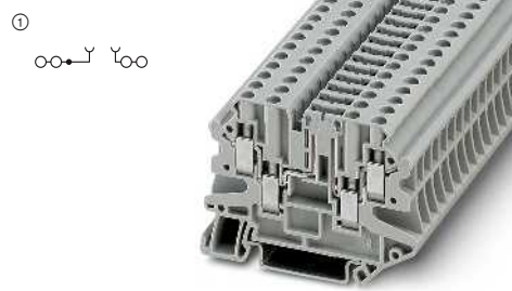
20 A, Trennklemme, 4 Anschlüsse
