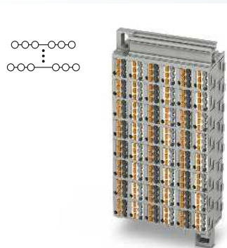
22 A, 48-polig, 288 Anschlüsse
