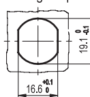
Drilling template
