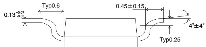
END VIEW
