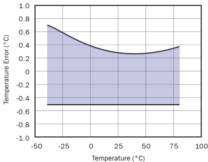
Temperature error vs Temperature
