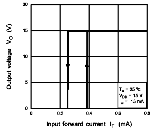
Fig. 12.2.4 V_O - I_F(IHYS)
