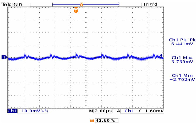
Figure 7: Output ripple & noise at 12Vin, 0.7525V/20A out
