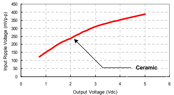
Figure 28: Input ripple voltage vs. output models, I_o = 20A ( C_{in} = 4x22\mu F ceramic capacitors at the input)
