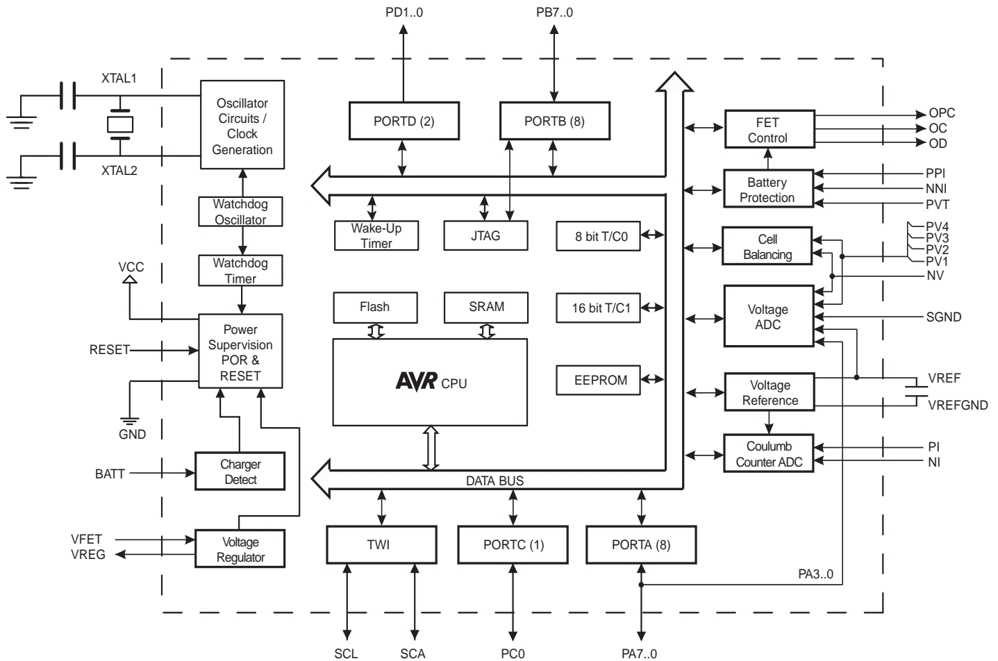
Figure 2-1. Block Diagram
