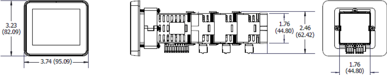
3.5 Inch Display
