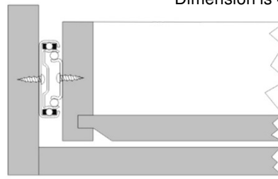
Installation Diagram
