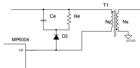
Figure 7—RCD snubber
