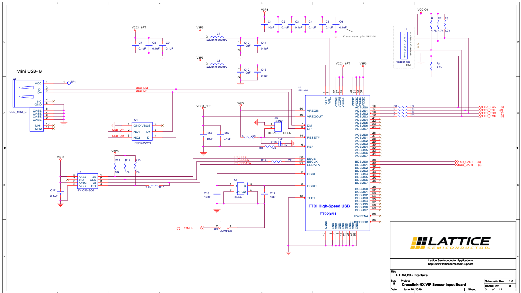
Figure A.3. FTDI/USB Interface
