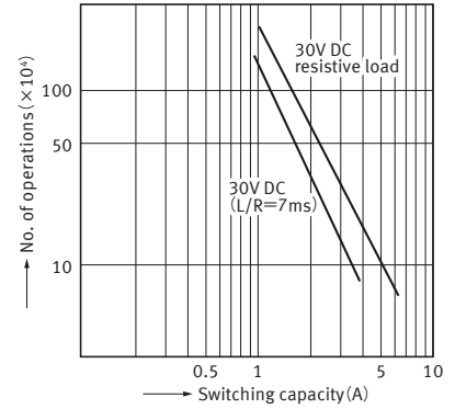
2-2. Switching life curve (1 Form A 1 Form B)
