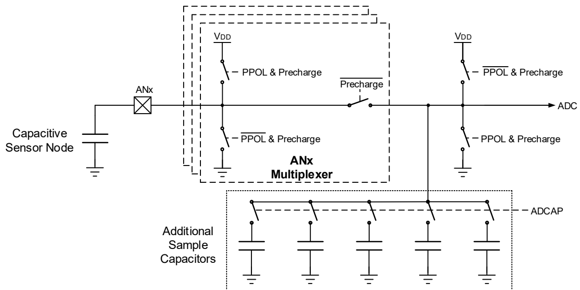
Figure 40-7. Hardware Capacitive Voltage Divider Block Diagram
