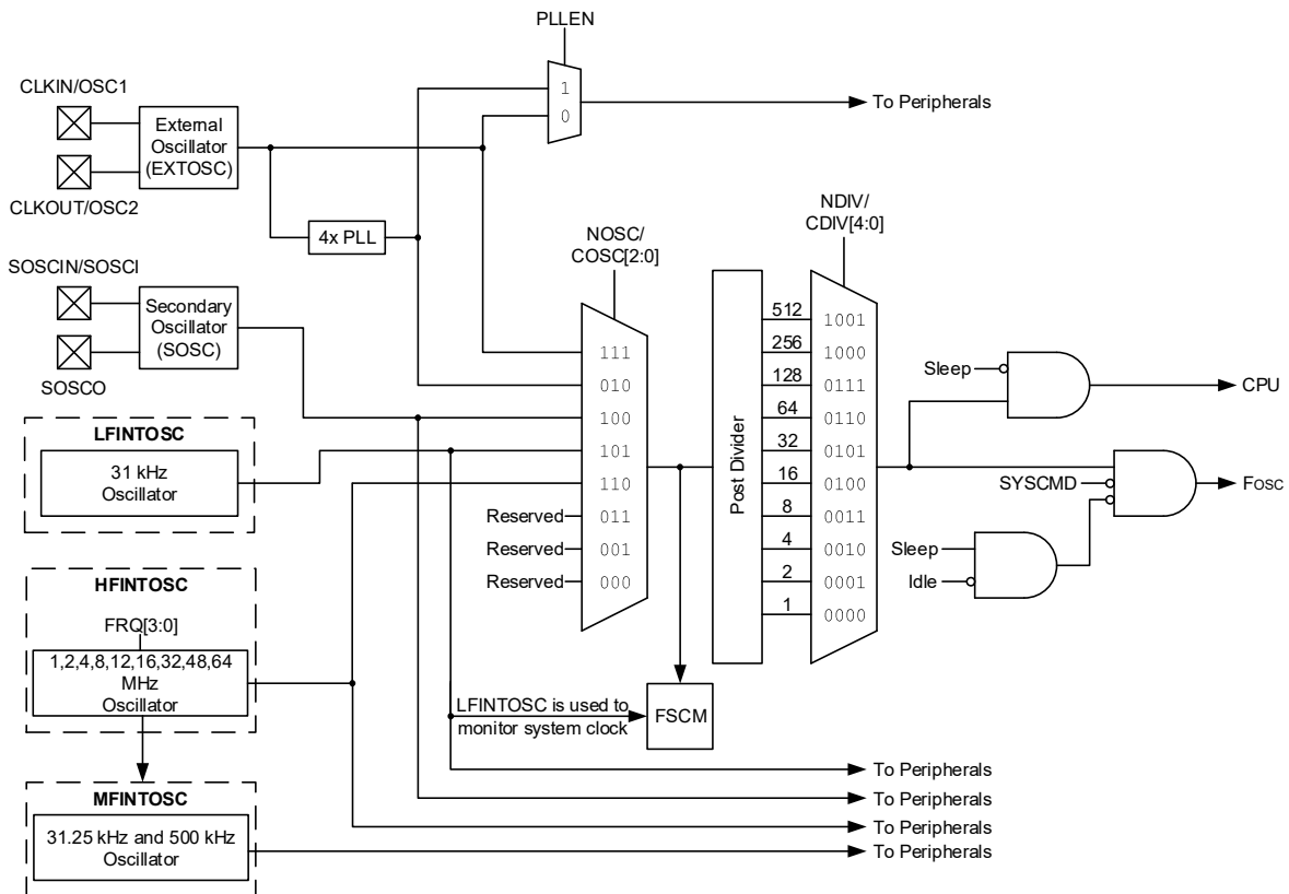
Figure 12-1. Clock Source Block Diagram
