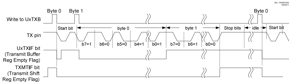
Figure 34-9. Manchester Timing
