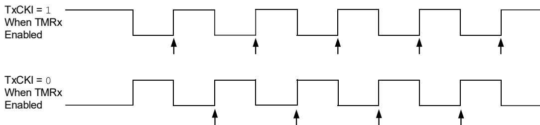
Figure 25-2. Timer1 Incrementing Edge
