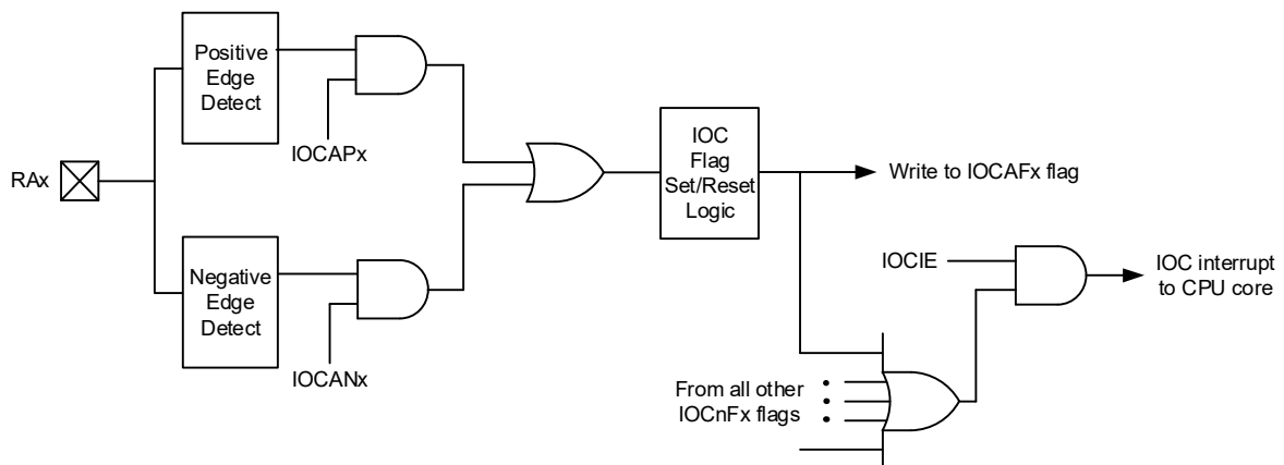
Figure 20-1. Interrupt-on-Change Block Diagram (PORTA Example)
