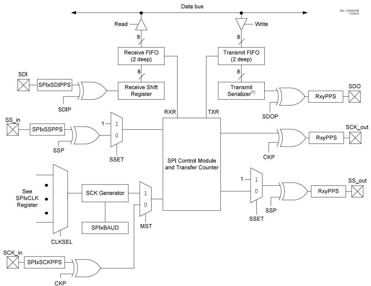
Figure 35-1. SPI Module Simplified Block Diagram
