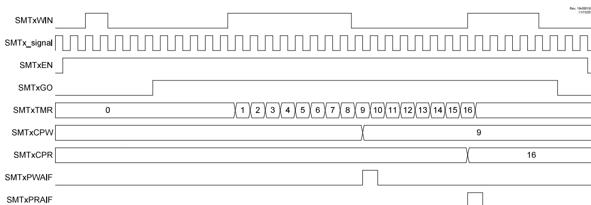
Figure 27-22. Windowed Counter Mode, Single Acquisition Timing Diagram
