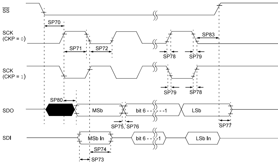
Figure 48-15. SPI Slave Mode Timing (CKE = 0)
