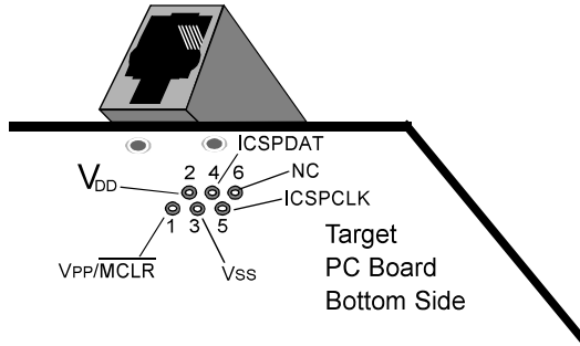
Figure 46-1. ICD RJ-11 Style Connector Interface
