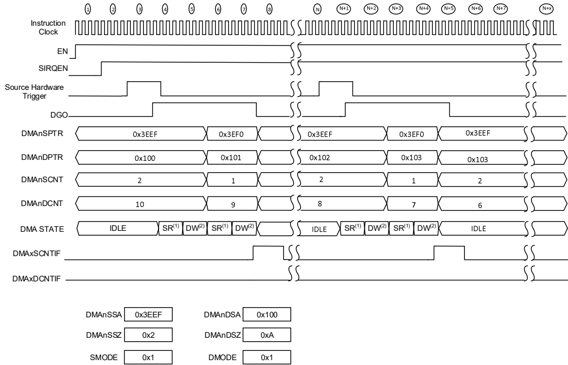
Figure 16-9. SFR Space to GPR Space Transfer
