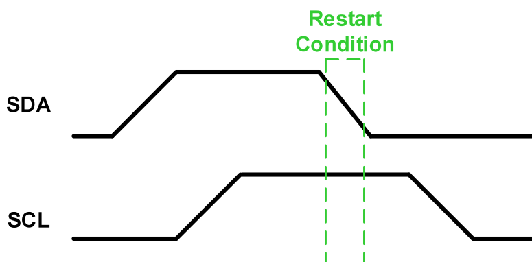
Figure 36-6. Restart Condition
