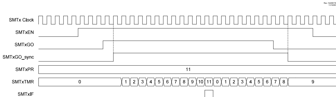
Figure 27-3. Timer Mode Timing Diagram
