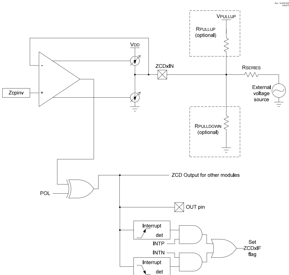
Figure 44-1. Simplified ZCD Block Diagram
