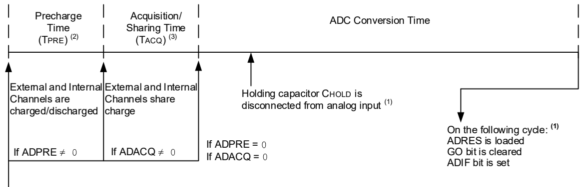
Figure 40-2. Analog-to-Digital Conversion Cycles
