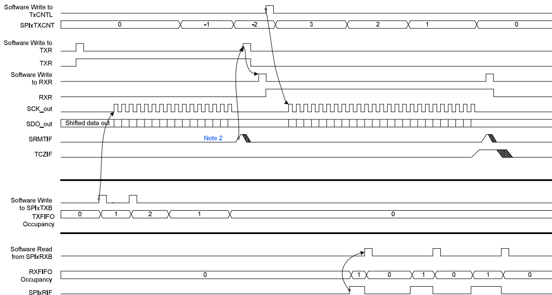
Figure 35-5. SPI Master Operation, Command+Read Data, TXR = 0, RXR = 1
