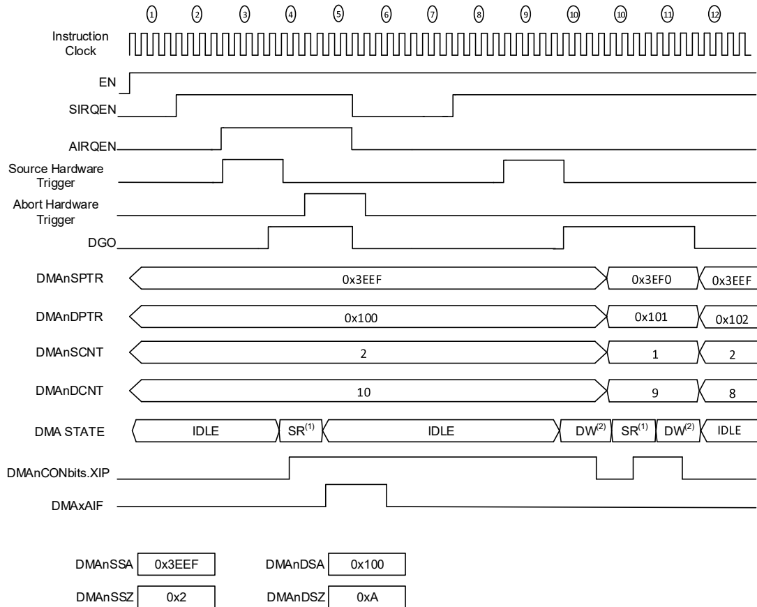
Figure 16-12. Abort During Message Transfer
