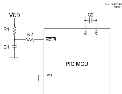
Figure 4-1. Recommended Minimum Connections
