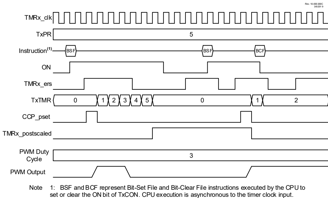
Figure 26-8. Edge-Triggered One-Shot Mode Timing Diagram (MODE = 'b01001)
