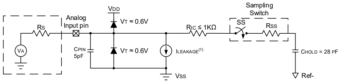
Figure 40-4. Analog Input Model
