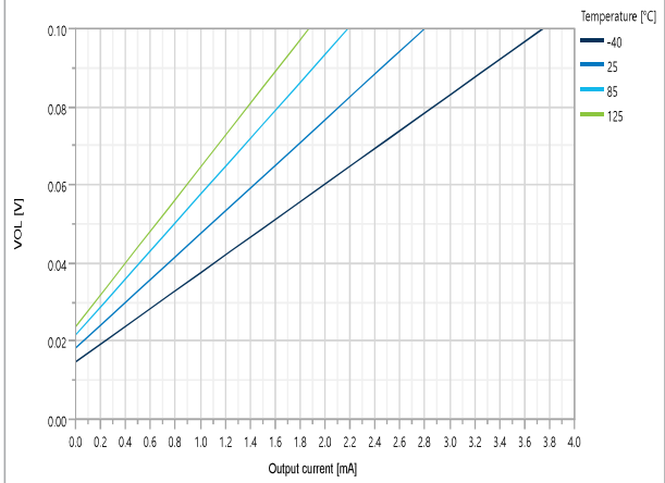
Figure 49-16. Output Short Circuit Current Over V_{DD} and Temperature
