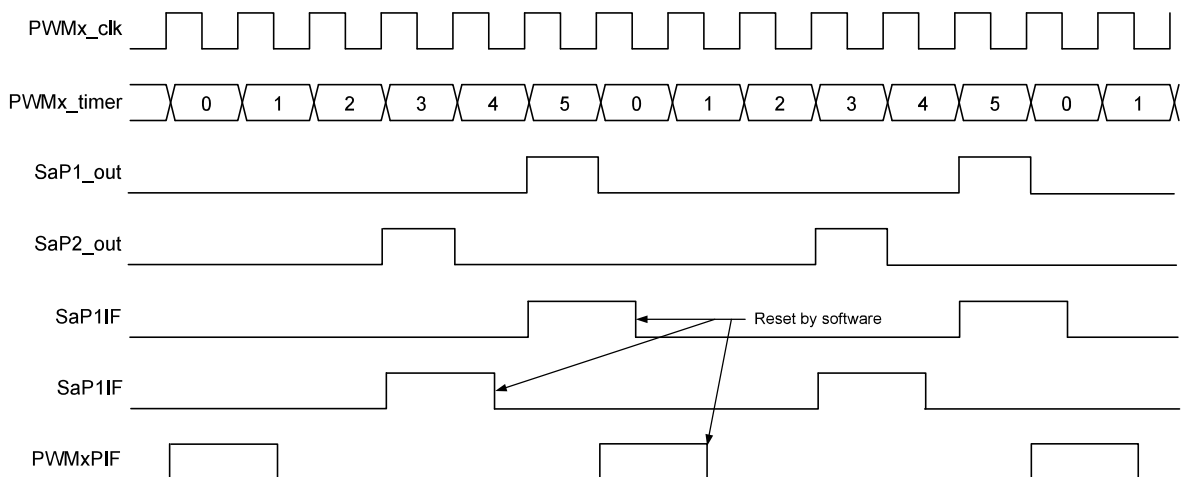
Figure 30-10. Pulsed Compare Timing Diagram
