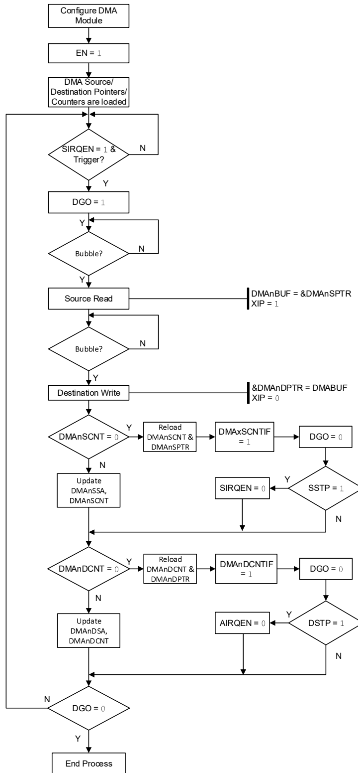
Figure 16-5. DMA Operation with Hardware Trigger
