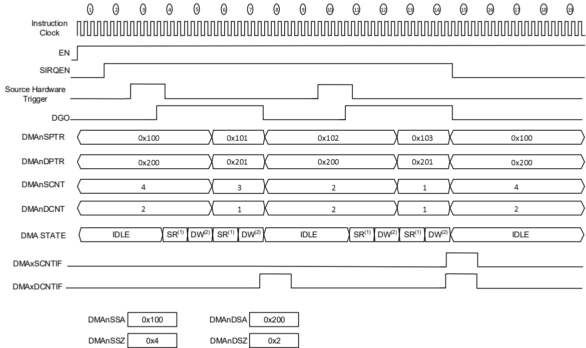
Figure 16-6. GPR-GPR Transactions with Hardware Triggers, SSTP = 1
