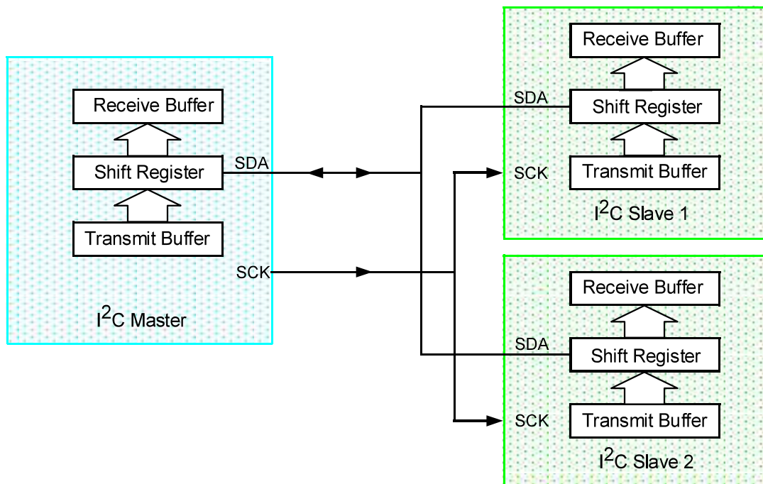
Figure 36-2. I 2 C Master-Slave Connections
