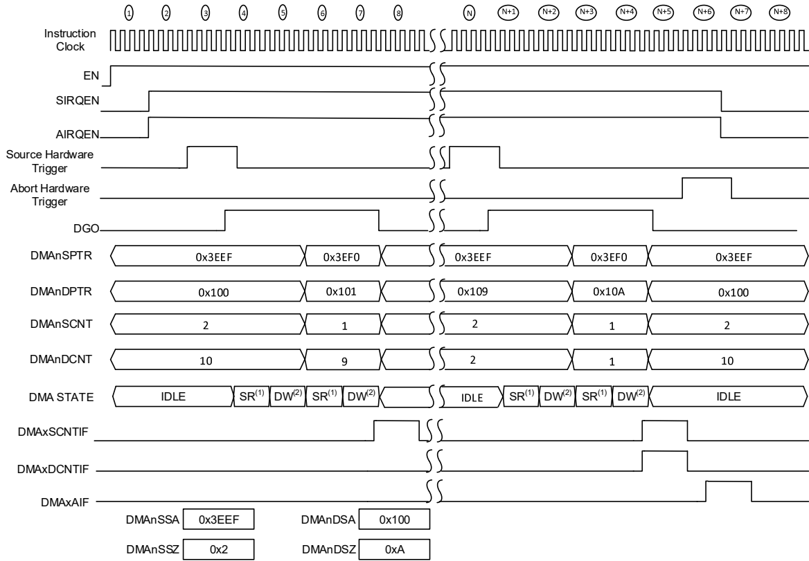
Figure 16-11. Abort at the End of Message
