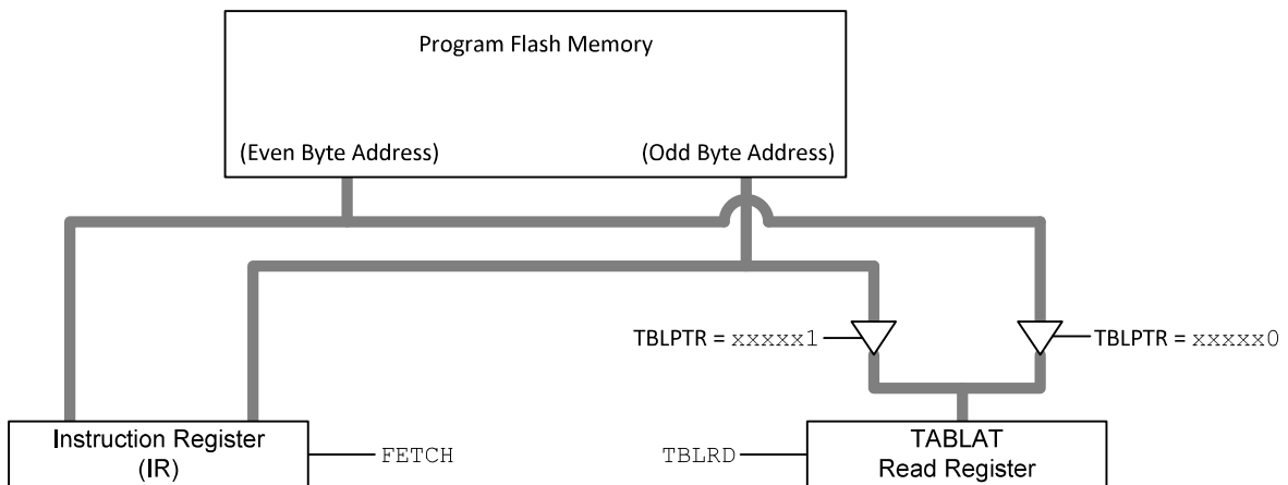
Figure 10-6. Reads from Program Flash Memory
