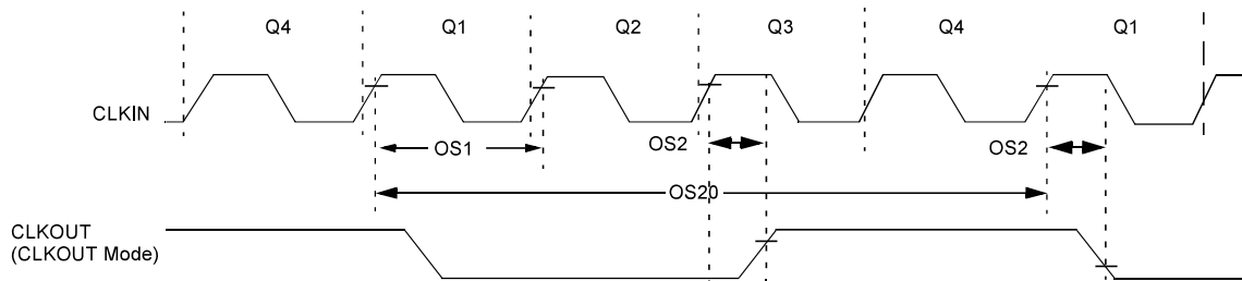
Figure 48-4. Clock Timing
