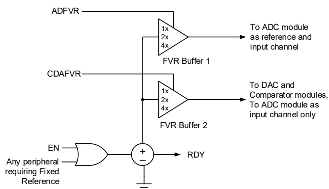
Figure 38-1. Fixed Voltage Reference Block Diagram
