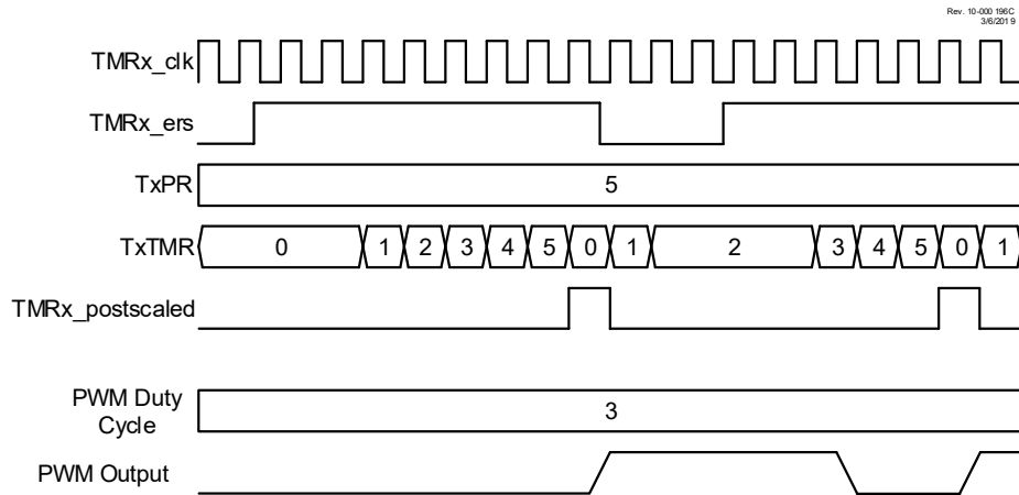
Figure 26-4. Hardware Gate Mode Timing Diagram (MODE = 'b00001 )
