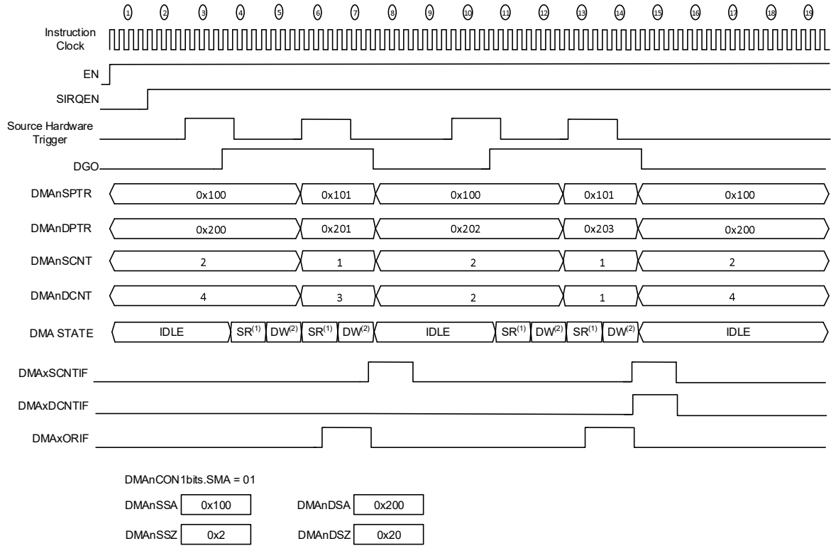
Figure 16-10. Overrun Interrupt
