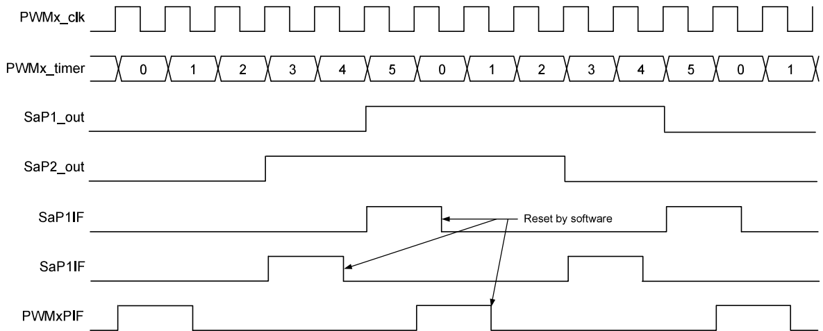
Figure 30-12. Toggled Compare Timing Diagram
