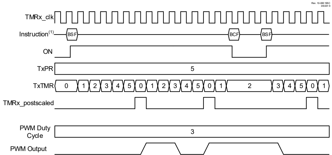
Figure 26-3. Software Gate Mode Timing Diagram (MODE = 'b000000)
