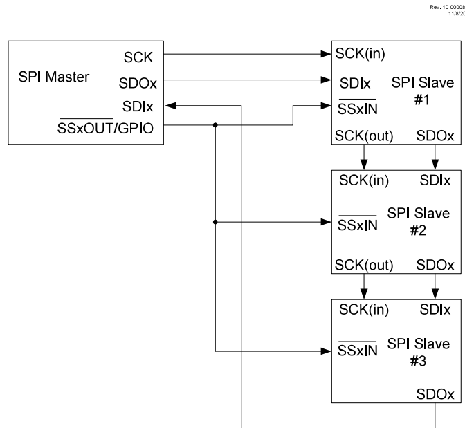
Figure 35-13. SPI Daisy-Chain Connection With Chained SCK
