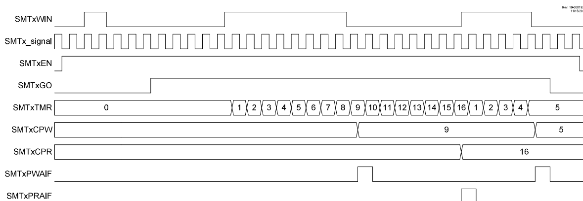
Figure 27-22. Windowed Counter Mode, Single Acquisition Timing Diagram
