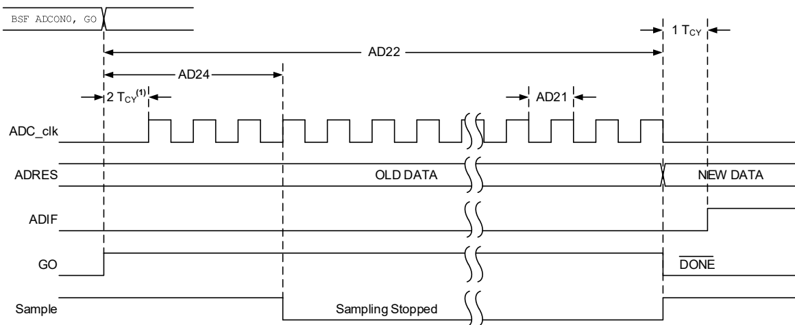
Figure 48-10. ADC Conversion Timing (ADC Clock from ADCRC)
