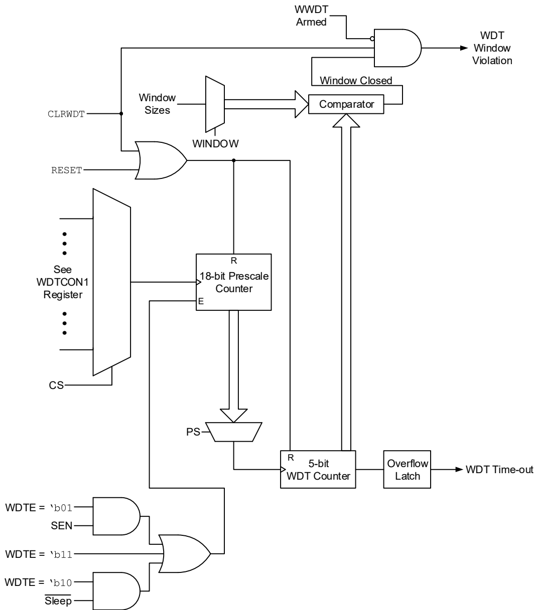
Figure 15-1. Windowed Watchdog Timer Block Diagram
