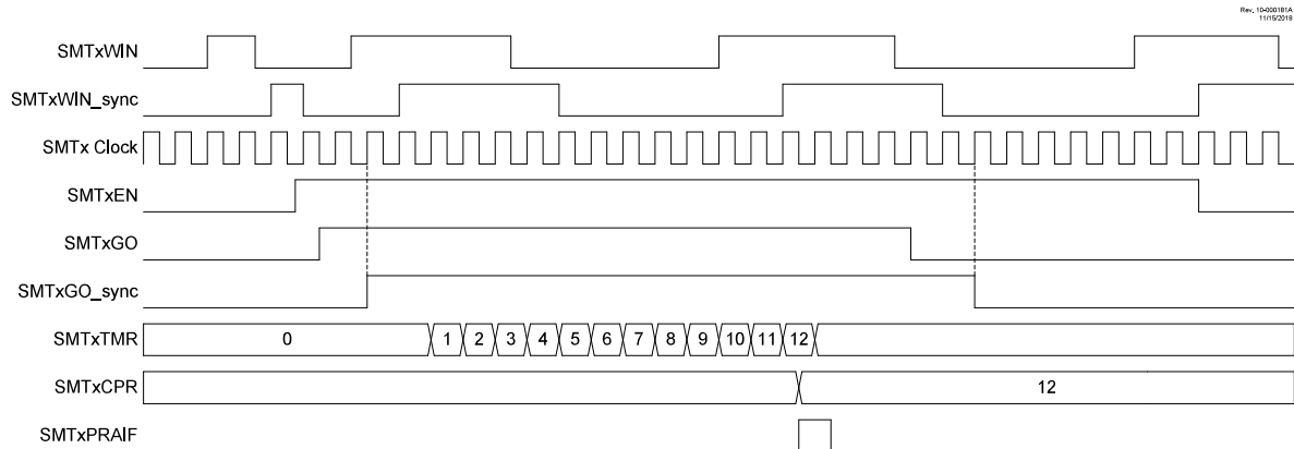
Figure 27-11. Windowed Measurement Mode, Single Acquisition Timing Diagram
