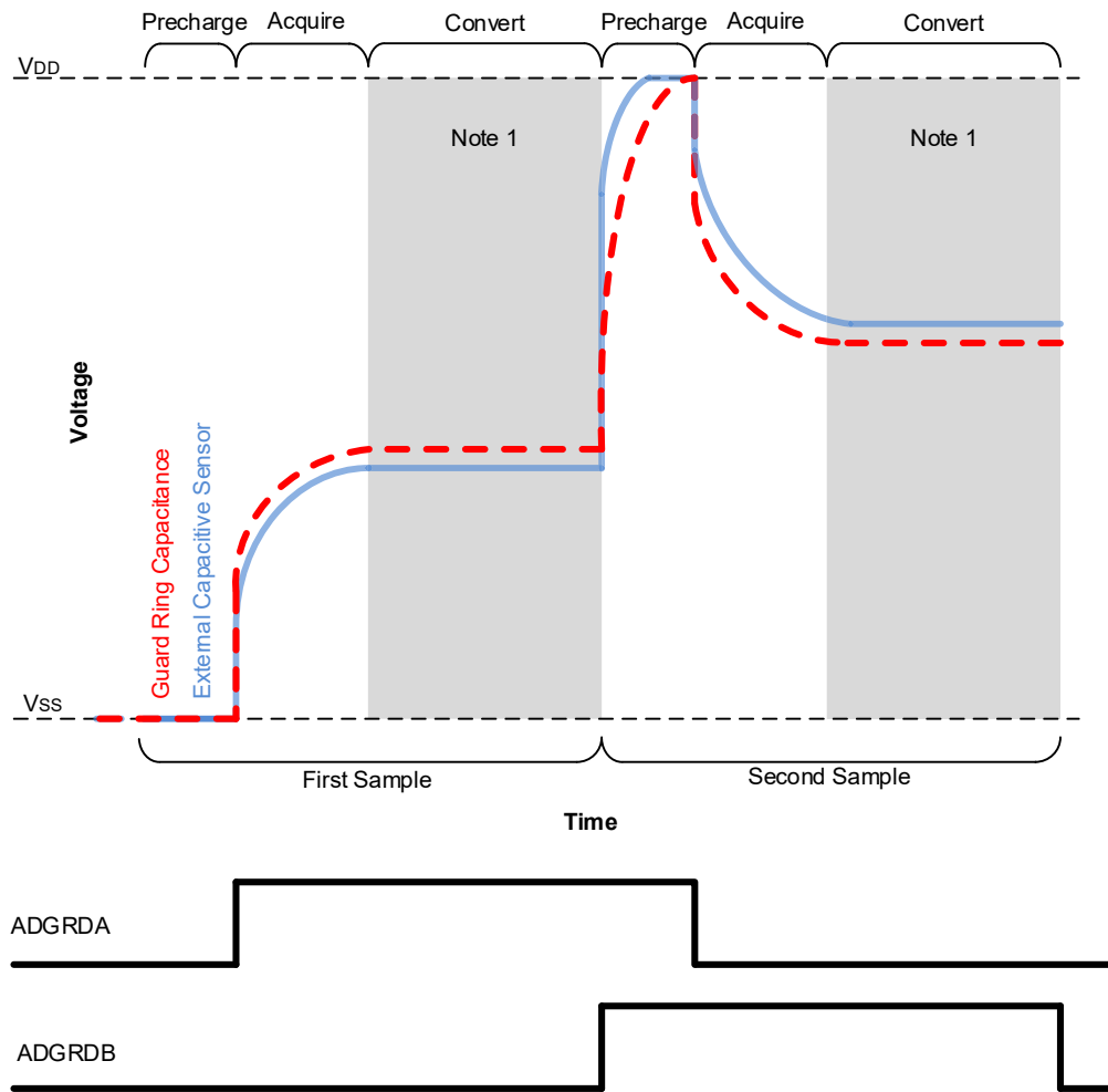
Figure 40-10. Differential CVD with Guard Ring Output Waveform
