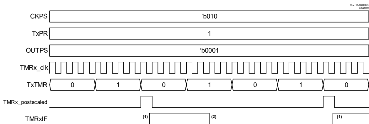
Figure 26-2. Timer2 Prescaler, Postscaler, and Interrupt Timing Diagram
