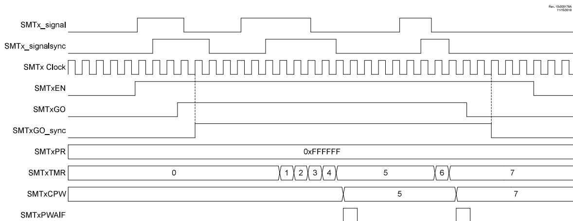
Figure 27-5. Gated Timer Mode, Single Acquisition Timing Diagram
