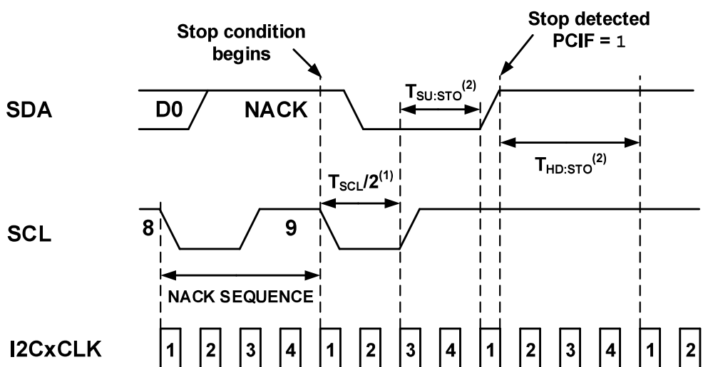
Figure 36-36. Stop Condition Timing
