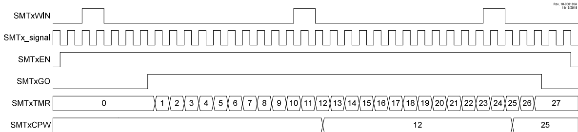
Figure 27-18. Counter Mode Timing Diagram
