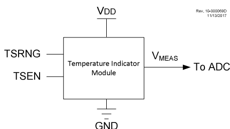
Figure 39-1. Temperature Indicator Module Block Diagram
