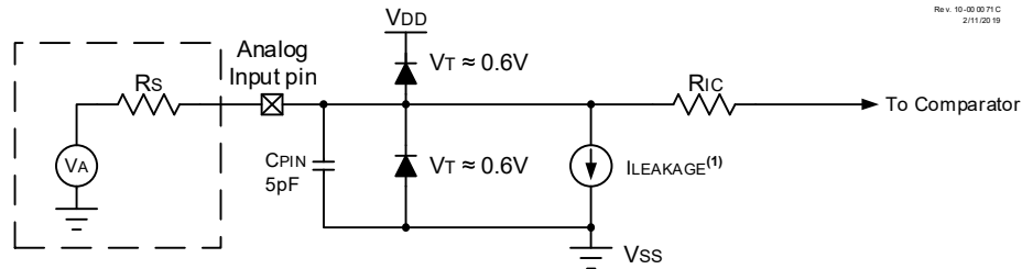
Figure 43-3. Analog Input Model
