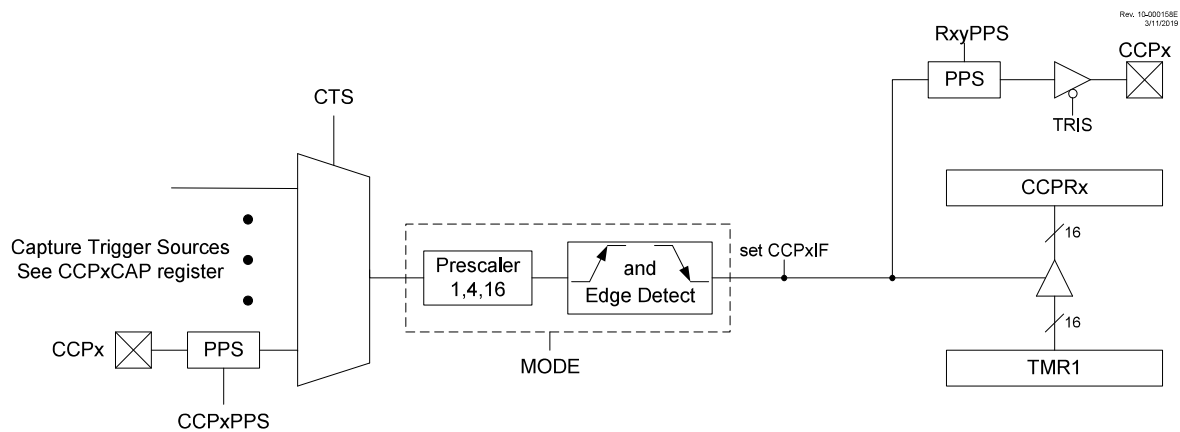
Figure 28-1. Capture Mode Operation Block Diagram
