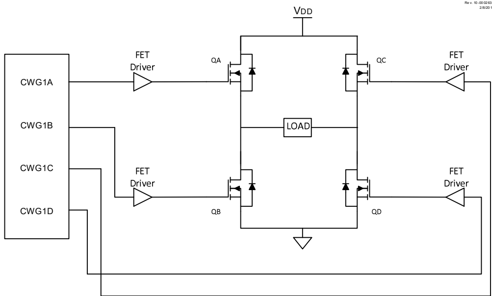
Figure 31-5. Example of Full-Bridge Application
