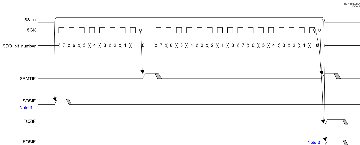
Figure 35-14. Transfer And Slave Select Interrupt Timing
