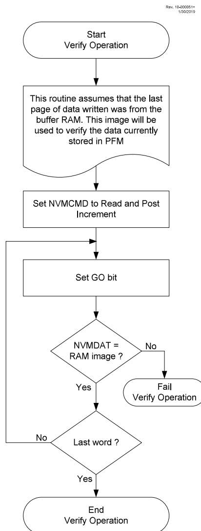
Figure 10-2. Program Flash Memory Write Verify Flowchart
