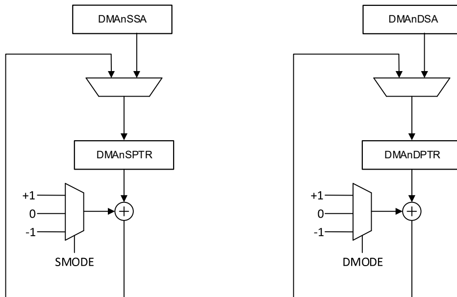
Figure 16-3. DMA Pointers Block Diagram
