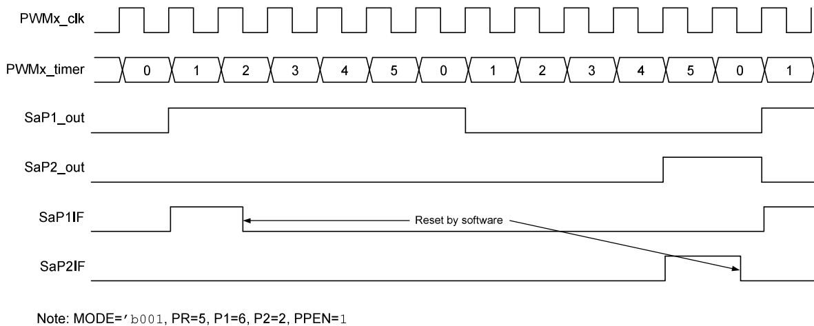
Figure 30-14. Right Aligned Push-Pull Mode Timing Diagram
