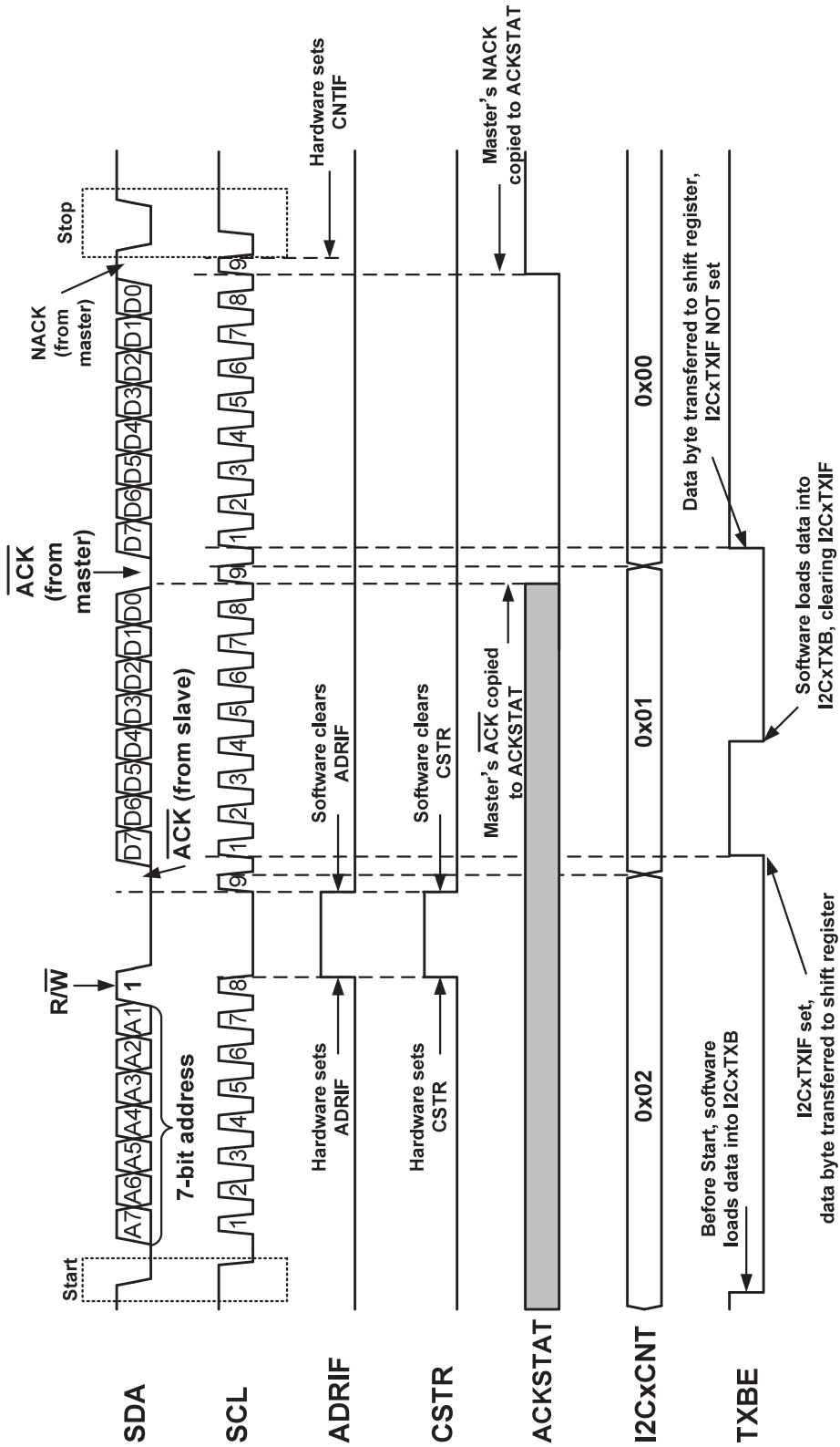
Figure 36-14. 7-Bit Slave Mode Transmission (ADRIE = 1)
