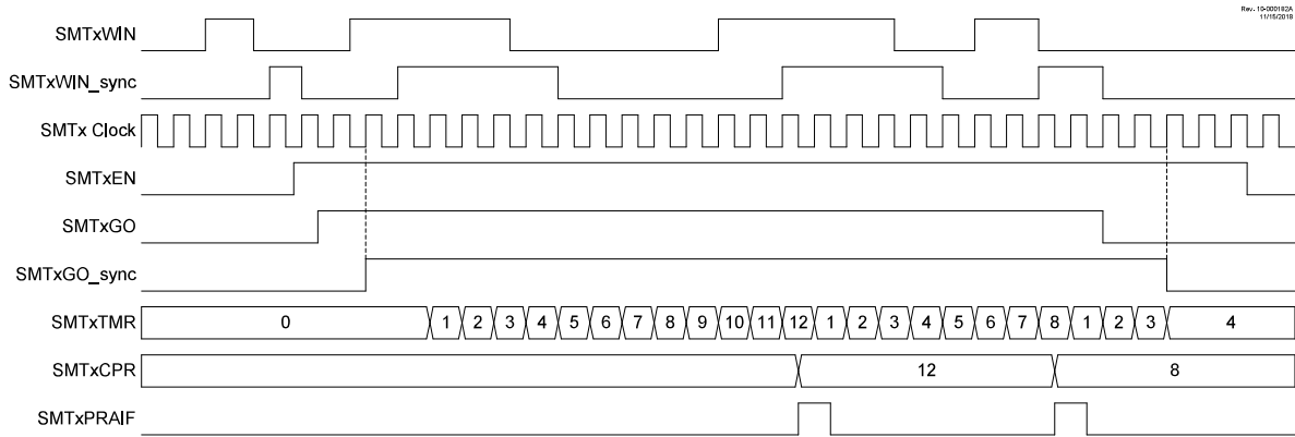
Figure 27-11. Windowed Measurement Mode, Single Acquisition Timing Diagram
