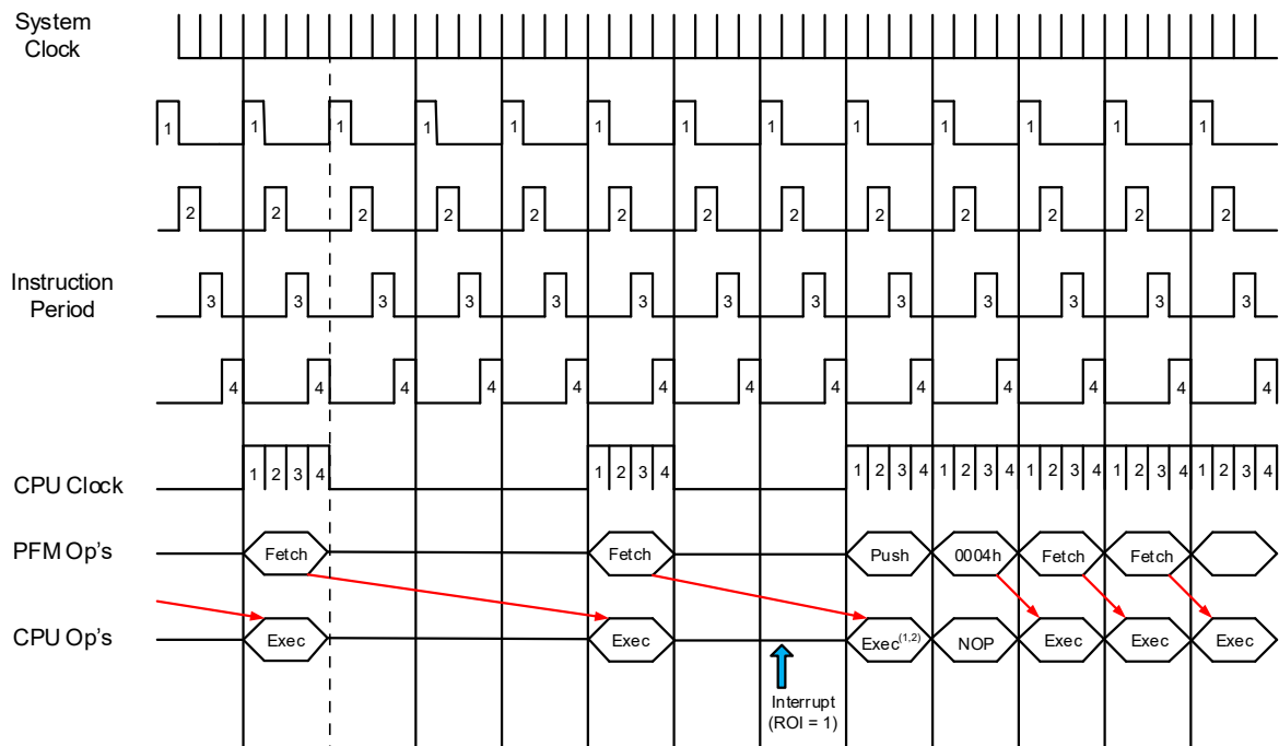
Figure 17-1. Doze Mode Operation Example
