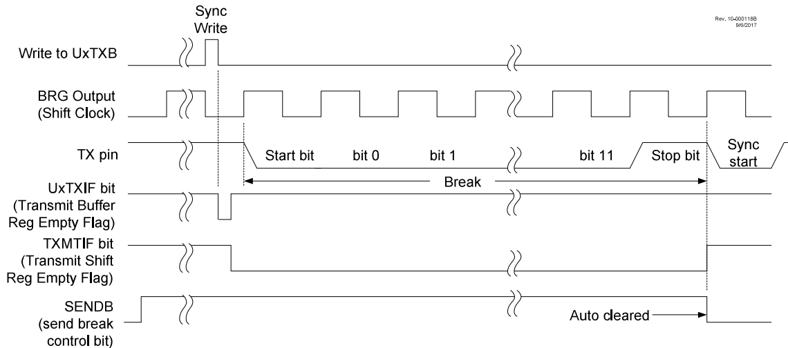
Figure 34-15. Send-Break Sequence
