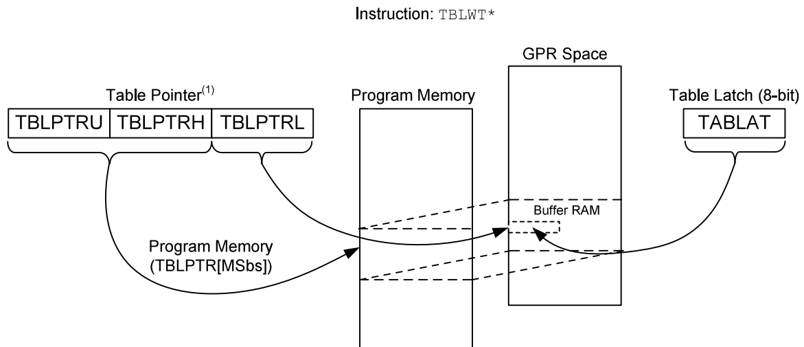
Figure 10-4. Table Write Operation
