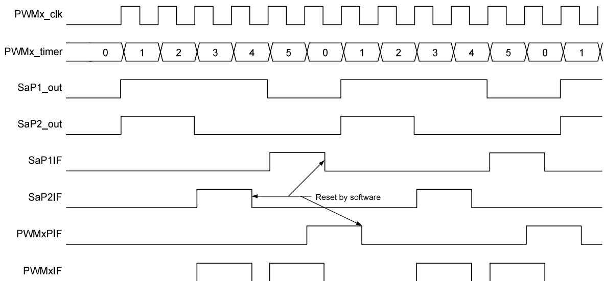
Figure 30-2. Left Aligned Timing Diagram
