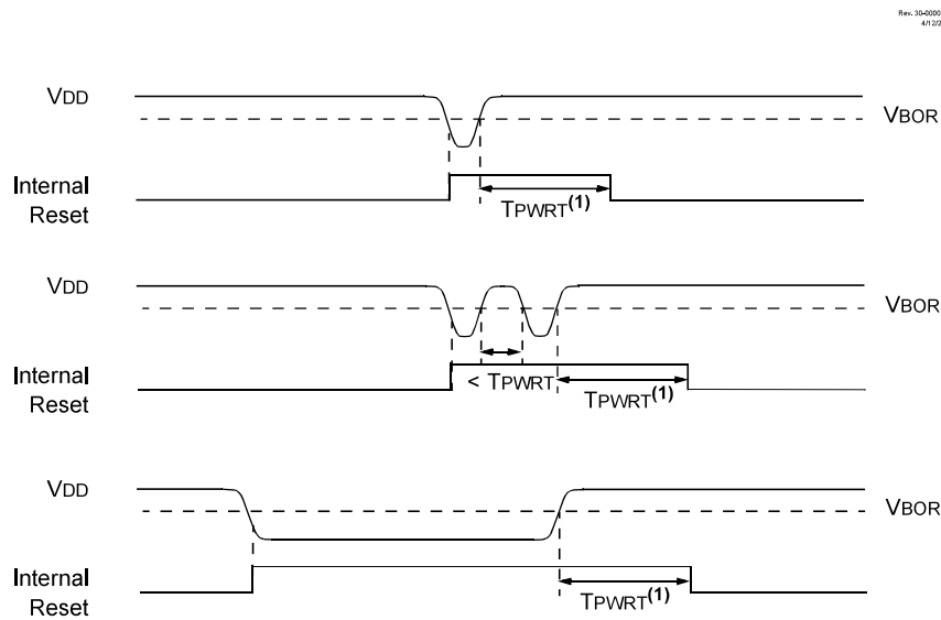
Figure 14-2. Brown-out Situations
