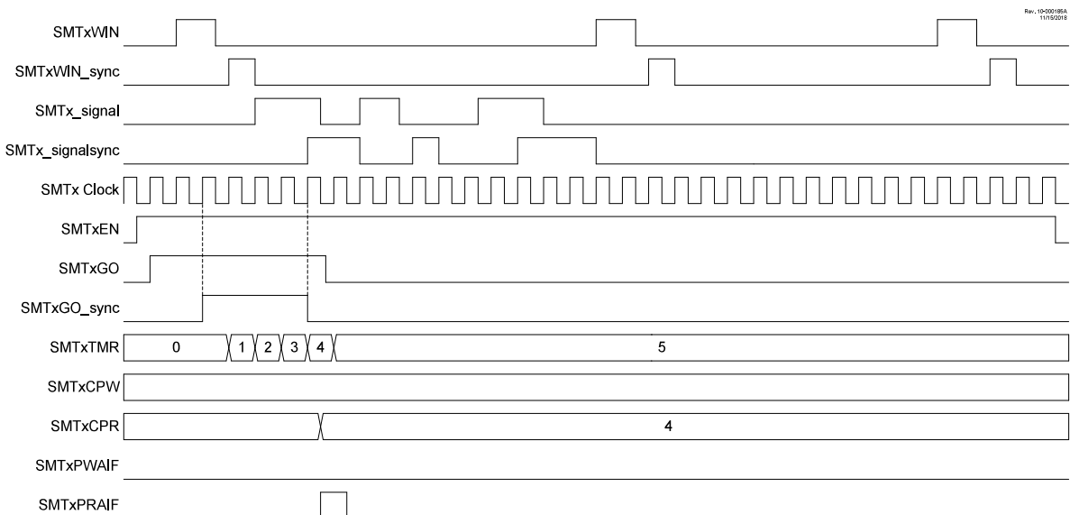
Figure 27-15. Time-of-Flight Mode, Single Acquisition Timing Diagram
