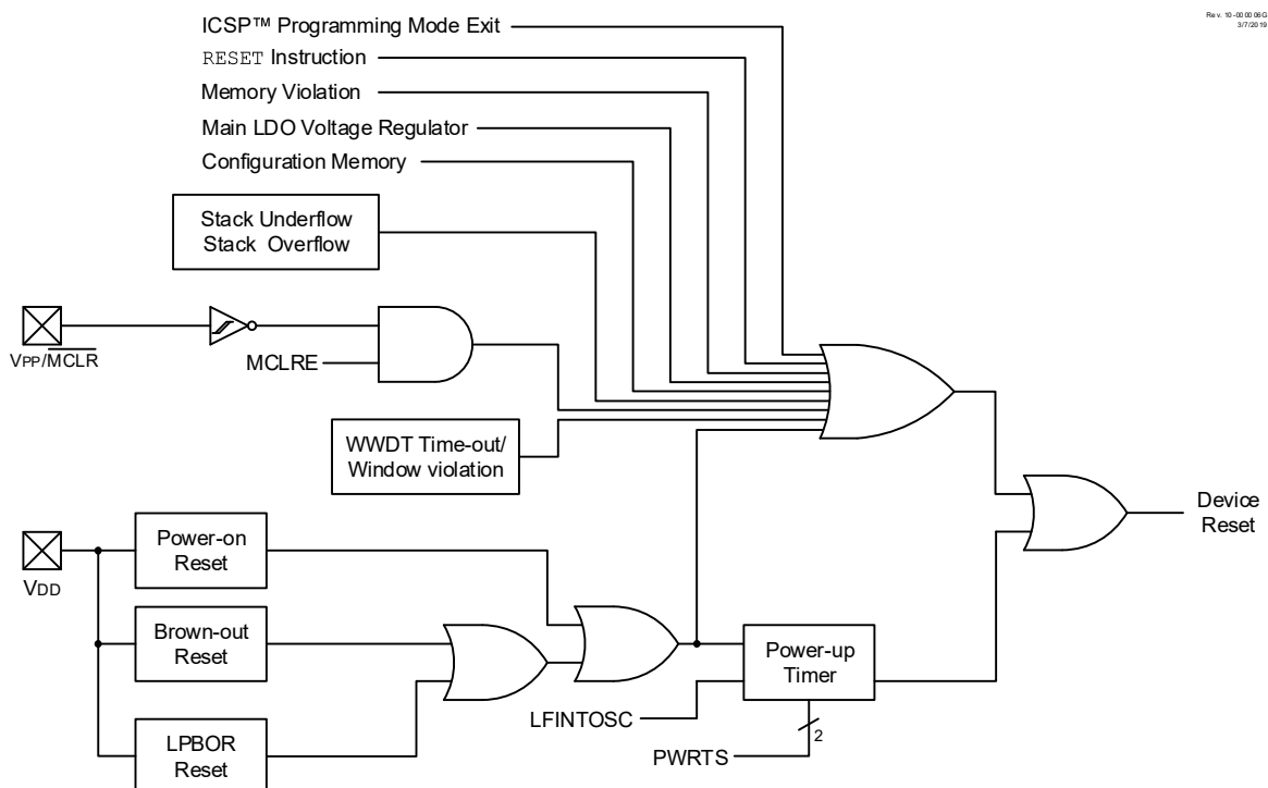
Figure 14-1. Simplified Block Diagram of On-Chip Reset Circuit
