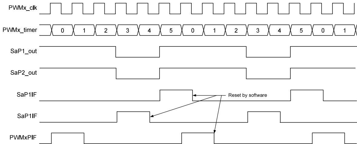
Figure 30-8. Variable Alignment Timing Diagram
