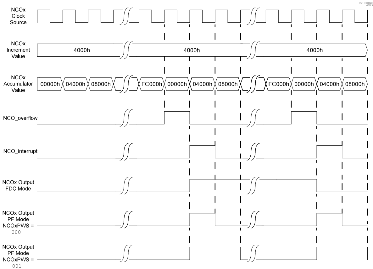
Figure 32-2. FDC Output Mode Timing Diagram
