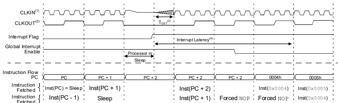
Figure 17-2. Wake-up From Sleep Through Interrupt
