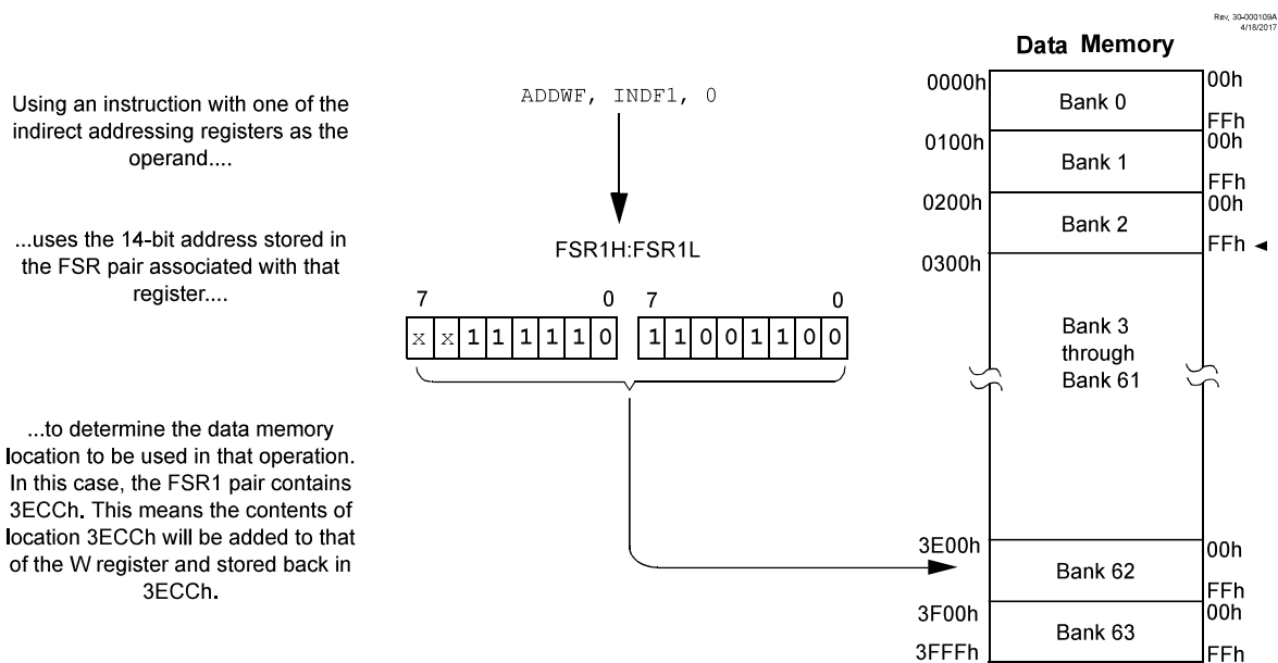
Figure 9-5. Indirect Addressing
