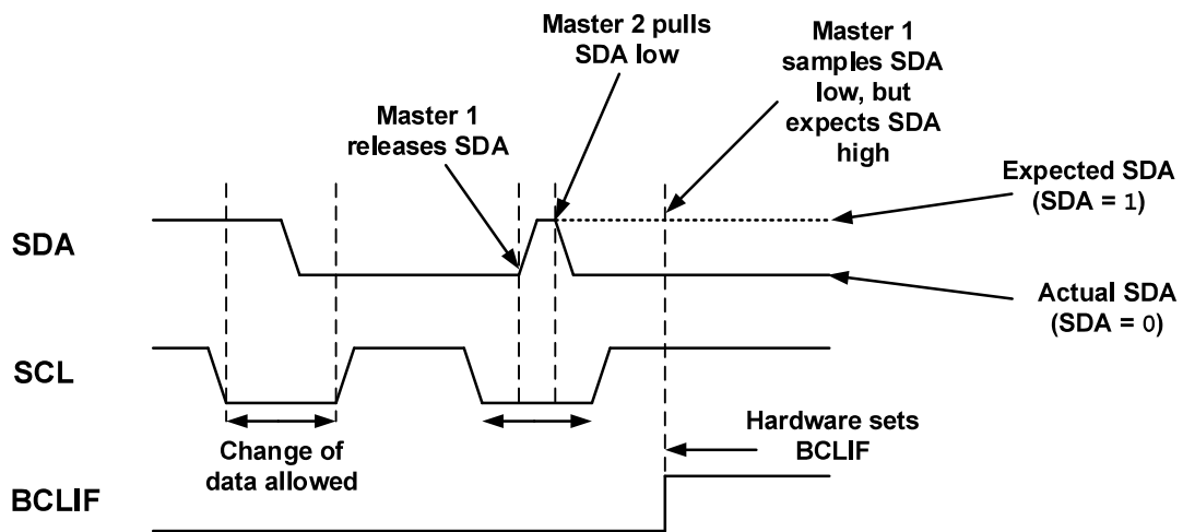
Figure 36-42. Bus Collision
