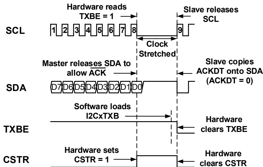
Figure 36-10. Transmit Buffer Clock Stretching
