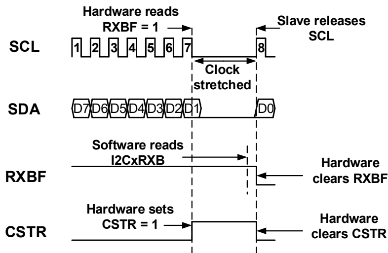
Figure 36-9. Receive Buffer Clock Stretching
