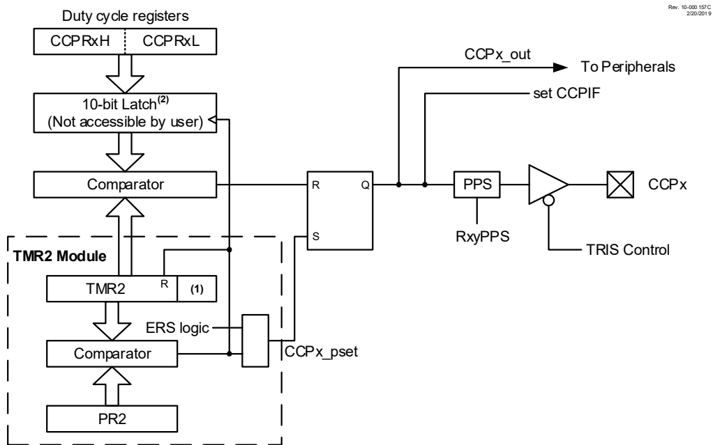
Figure 28-4. Simplified PWM Block Diagram
