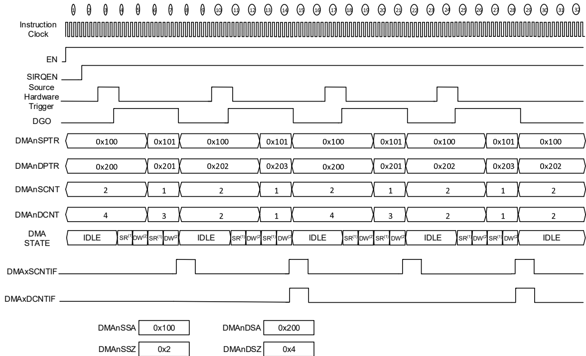
Figure 16-8. GPR-GPR Transactions with Hardware Triggers, SSTP, DSTP = 0
