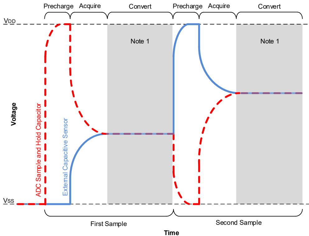
Figure 40-8. Differential CVD Measurement Waveform
