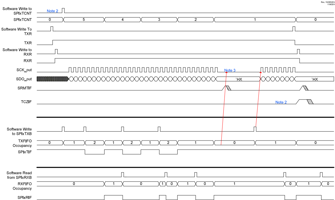
Figure 35-3. SPI Master Operation - Data Exchange RXR = 1, TXR = 1
