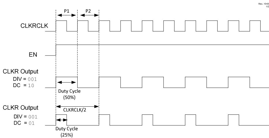
Figure 23-2. Clock Reference Timing
