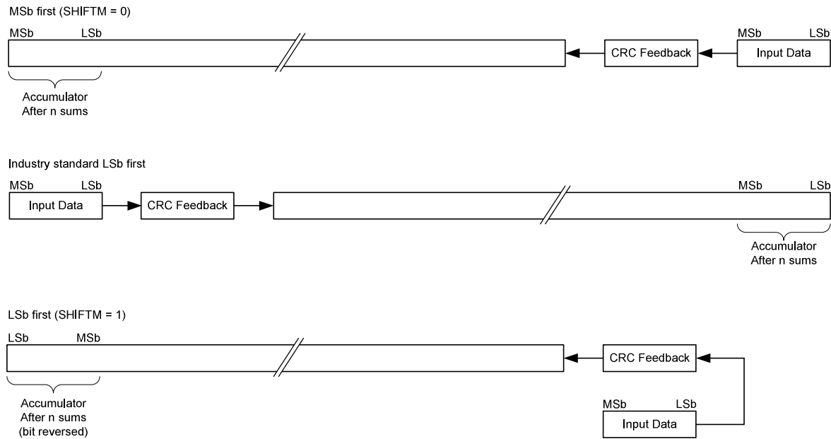
Figure 13-1. CRC Process
