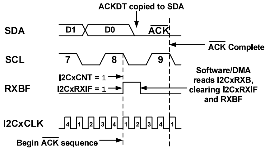
Figure 36-33. Acknowledge ( \overline{\text{ACK}} ) Sequence Timing
