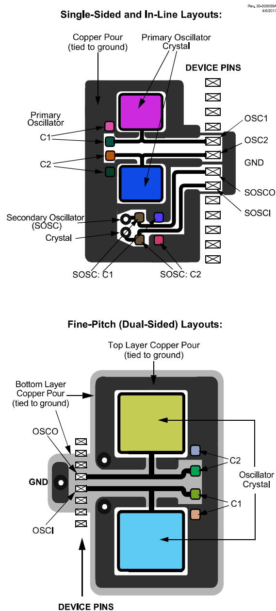
Figure 4-3. Suggested Placement of the Oscillator Circuit
