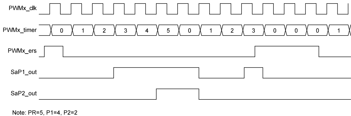
Figure 30-16. Left Aligned Mode with ERSNOW = 0
