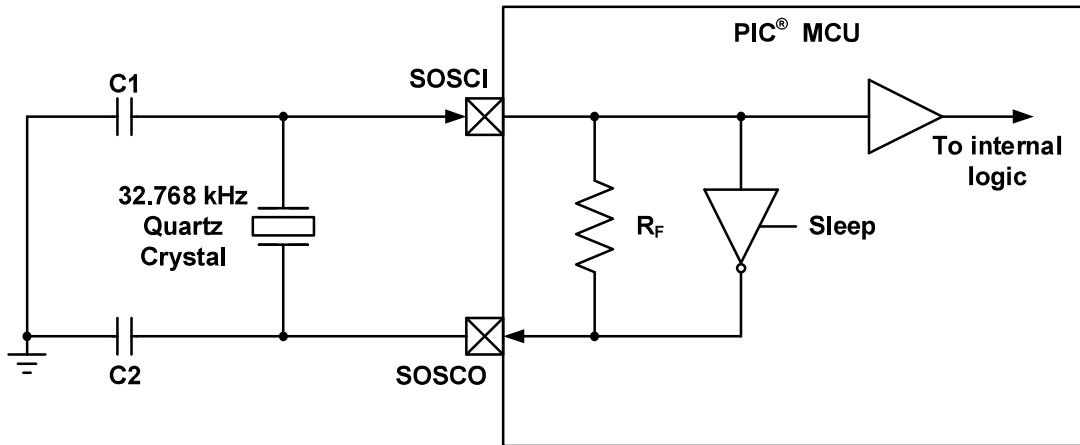
Figure 12-6. SOSC 32.768 kHz External Clock Operation
