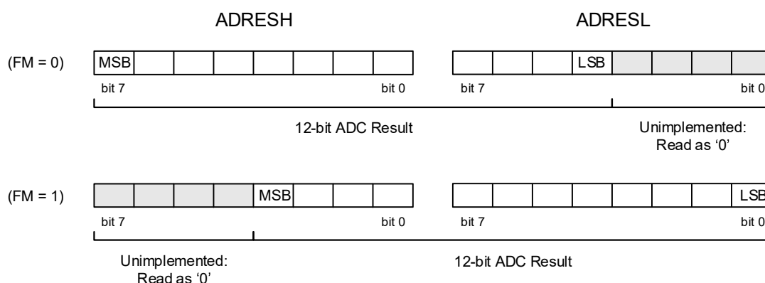
Figure 40-3. 12-Bit ADC Conversion Result Format
