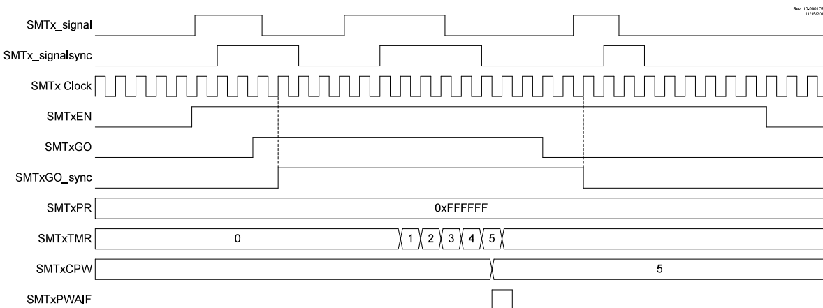
Figure 27-5. Gated Timer Mode, Single Acquisition Timing Diagram
