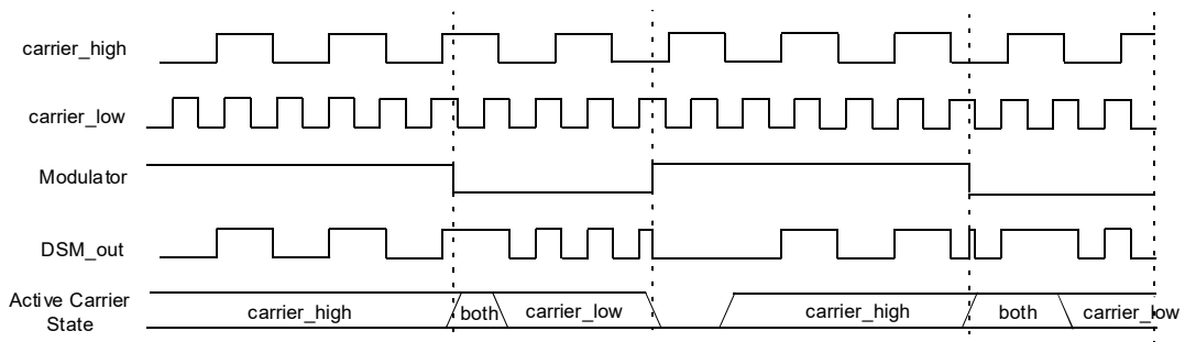
Figure 33-5. Carrier Low Synchronization (CHSYNC = 0, CLSYNC = 1)
