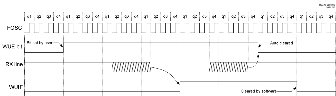
Figure 34-13. Auto Wake-Up Timing During Normal Operation
