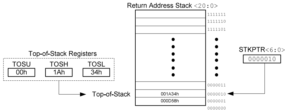
Figure 9-2. Return Address Stack and Associated Registers
