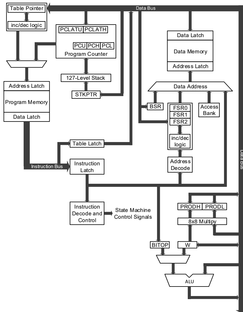
Figure 7-1. Family Block Diagram
