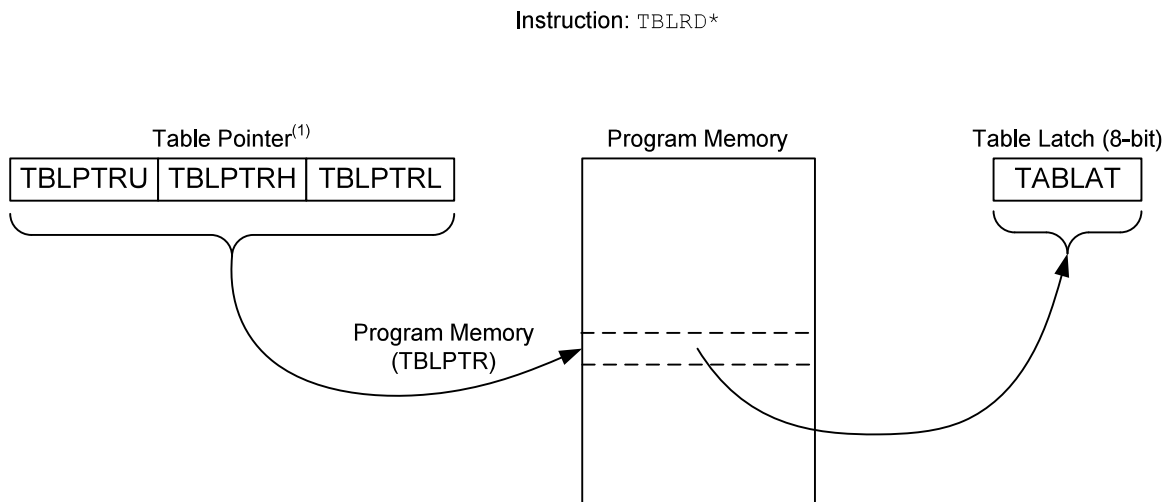
Figure 10-3. Table Read Operation
