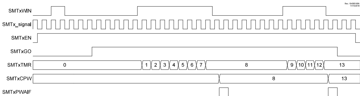
Figure 27-20. Gated Counter Mode, Single Acquisition Timing Diagram
