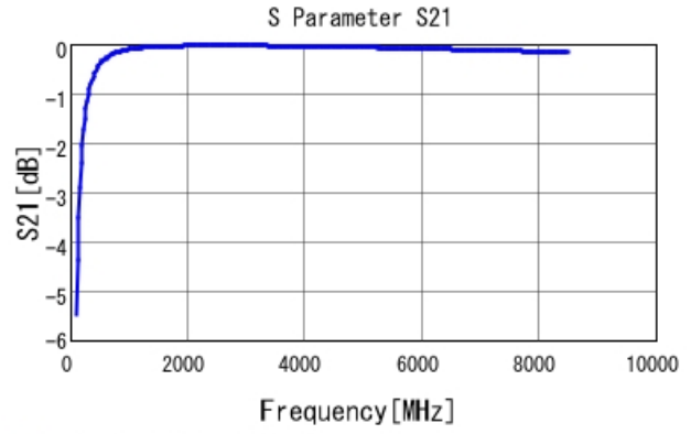
■ GRM0335C1H100JA01 S21 DCOV, 25degC
