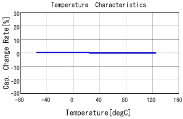
■ GRM0335C1H100JA01 C-Temp. capchange, DCOV, AC1Vrms
