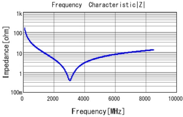
■ GRM0335C1H100JA01 |Z| DC0V, 25degC
