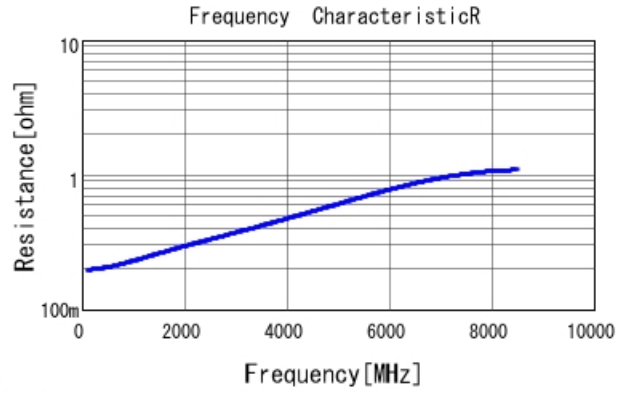
■ GRM0335C1H100JA01 R DC0V, 25degC
