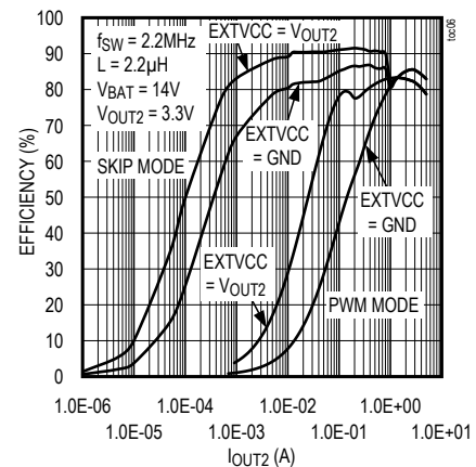
BUCK2 EFFICIENCY
