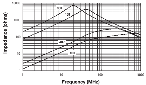
Impedance Characteristics
