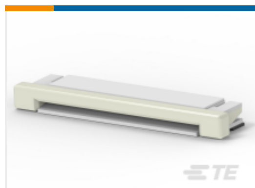
TE Part #1734742-6 0.5mm FPC Connectors
