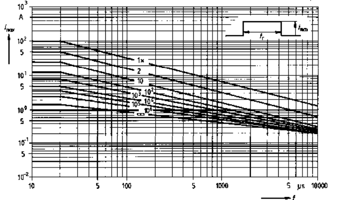
Fig. 12 Curve Giving The Max. Number Of Overload Pulses Regarding Their Duration For The Overvoltage Protection Of The Status Outputs
