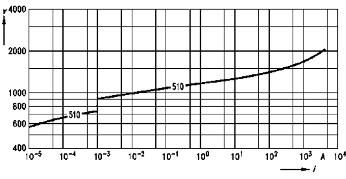
Overvoltage Protection Characteristic (Varistors)
