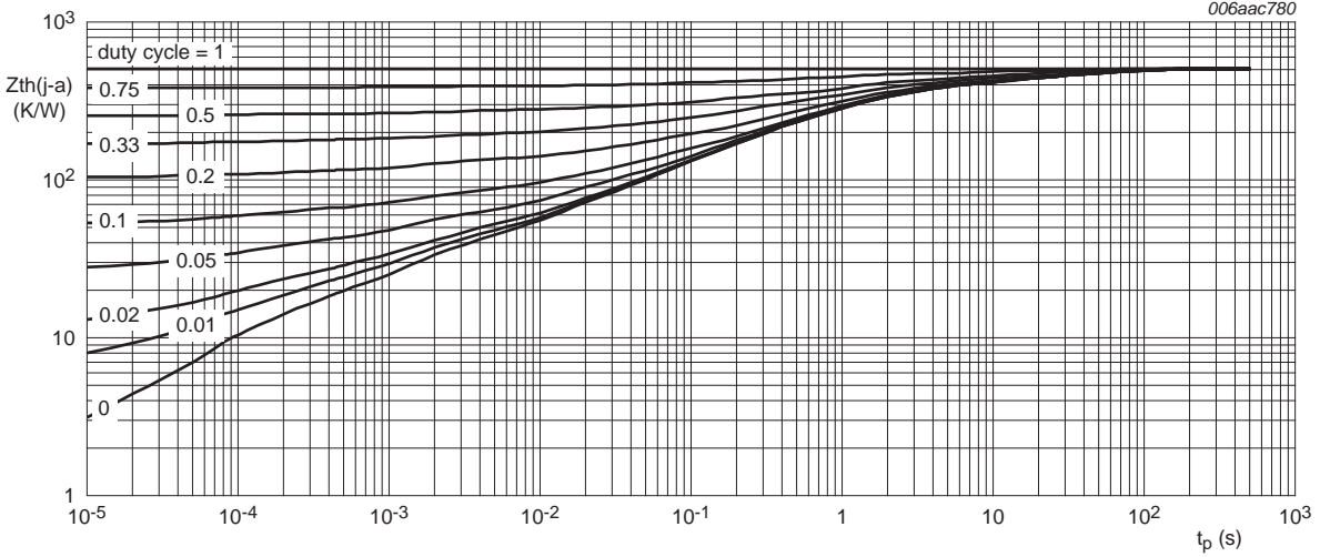
Fig 5. Transient thermal impedance from junction to ambient as a function of pulse duration for PDTC143EU (SOT323); typical values
