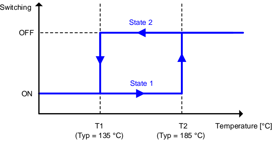
Figure 13. Thermal Shutdown Function
