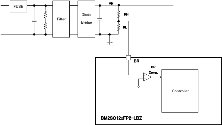
Figure 14. BR UVLO Function
