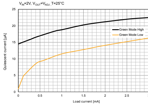
Figure 24. Quiescent current vs. load current (light load)
