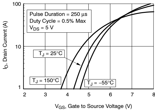
Figure 3. Transfer Characteristic
