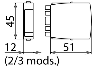
Dimension drawing BXT ML4 BE 48
