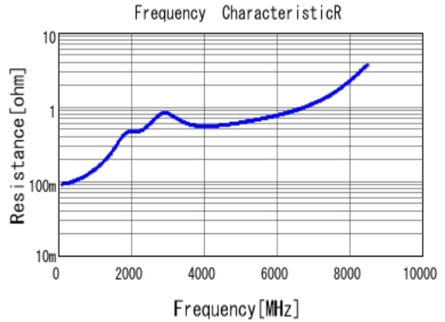
■ GRM0335C1E151JA01 R DC0V, 25degC
