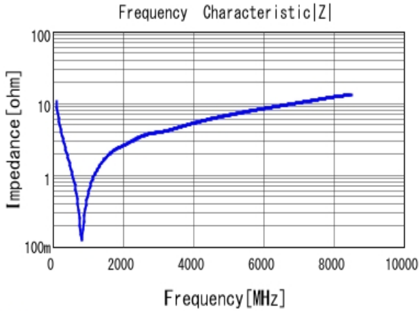
■ GRM0335C1E151JA01 |Z| DC0V, 25degC
