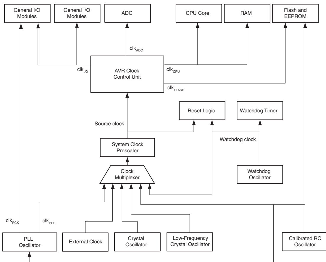
Figure 6-1. Clock Distribution
