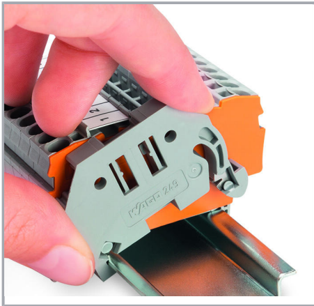
Snap-on mounting
